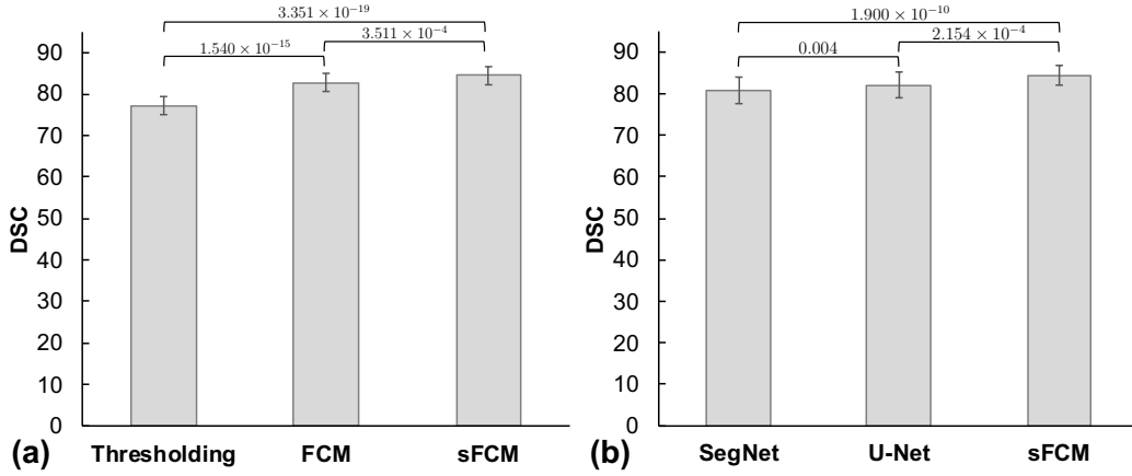
Figure 7: DSC values achieved by: (a) interactive methods based on classic image processing techniques (namely, thresholding, FCM and sFCM); (b) CNN-based approaches compared against the proposed sFCM method (in a 5-fold CV scheme). The bar graph and error bars denote the average value and the standard deviation DSC values, respectively. The p -values, obtained from the statistical validation procedure, are shown at the top of the bars as brackets. The Wilcoxon rank-sum test for pairwise result comparison was used with the alternative hypothesis that the samples do not have equal medians of DSC values. A significance level of \alpha = 0.05 with a correction using the Bonferroni–Holm method for multiple comparisons.
