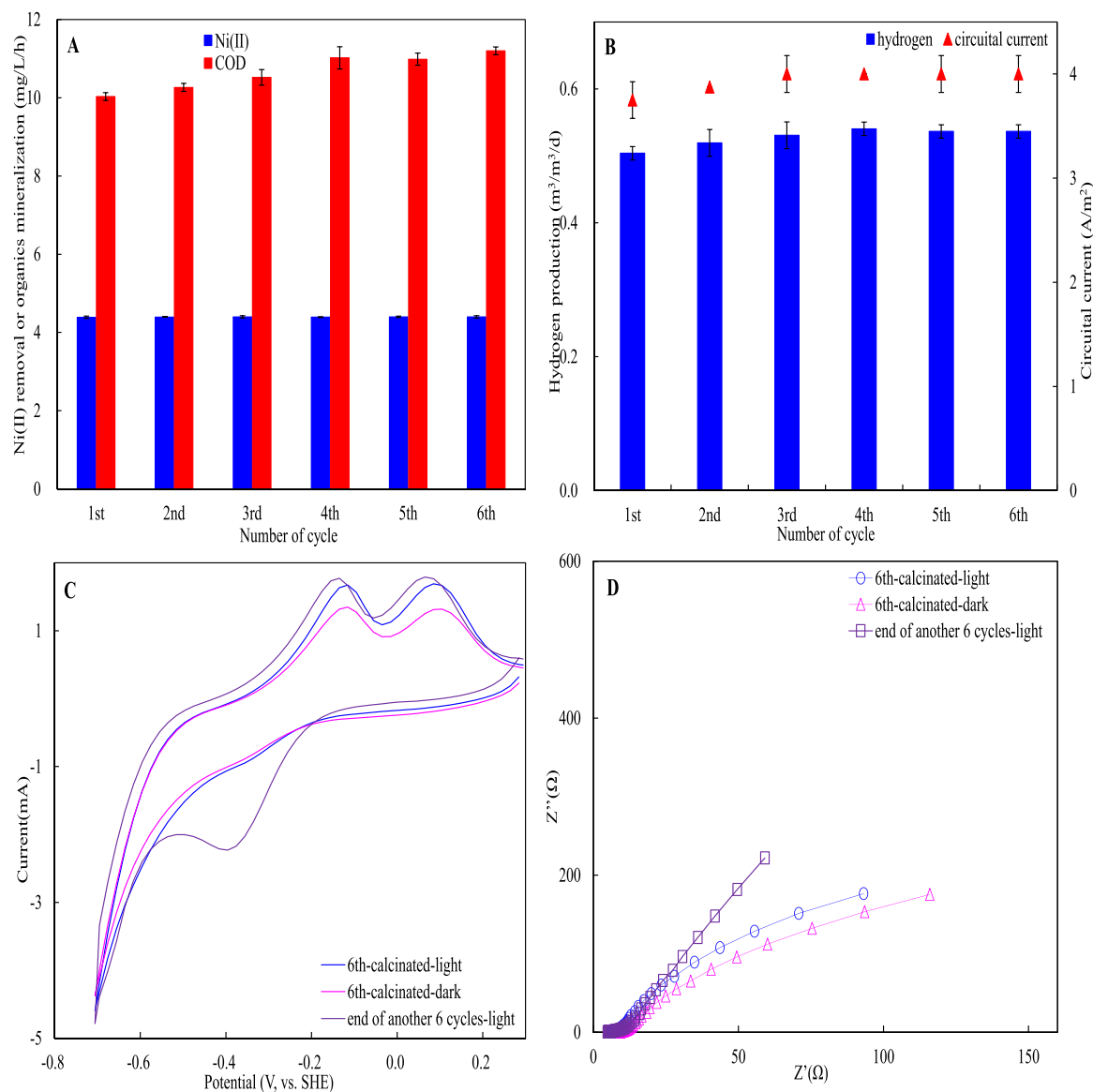
Fig. 5. Assessment of Ni(II) removal and organics mineralization (A), hydrogen production and circuit current (B), CV tests (C), and Nyquist plots of EIS spectra (D) on the calcinated ZnFe 2 O 4 /g-C 3 N 4 cathodes for ETW treatment.
