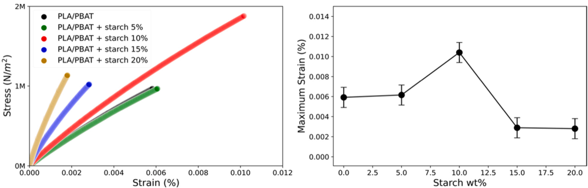
Fig. 7. left panel: stress-strain plot for PLA/PBAT/starch composites at various starch wt%. Right panel: maximum strain beared by the composites under investigation as a function of starch wt%.
