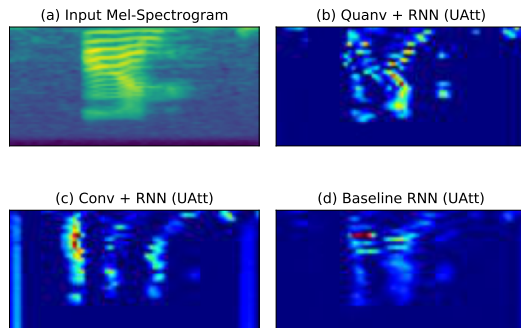
Fig. 6: Interpretable neural saliency results by class activation mapping [32] over (a) Mel spectrogram features with audio transcription of "on"; (b) a 2 \times 2 quantum convolution layer followed by \text{RNN}_{\text{UAtt}} ; (c) a well-trained 2 \times 2 neural convolution layer followed by \text{RNN}_{\text{UAtt}} , and (d) baseline \text{RNN}_{\text{UAtt}} .
