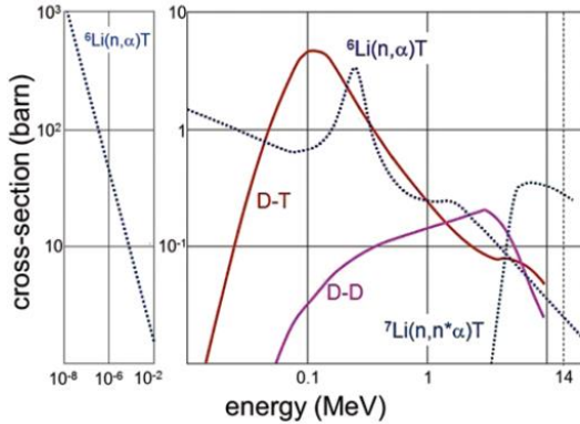
Fig. 1: Cross sections of the {}^6\text{Li} and {}^7\text{Li} T breeding reactions as a function of the impacting neutron energy. D-D and D-T cross-sections as a function of the plasma energy are reported as well. Figure is taken from [13].
