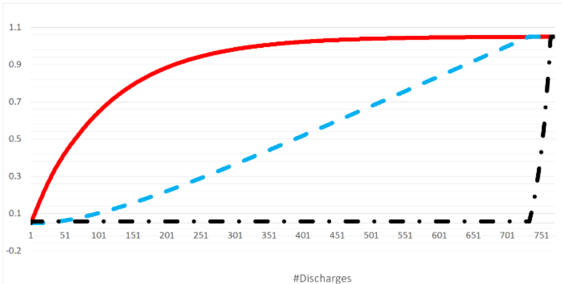
Fig. 5: Number of discharges needed to achieve the target state, i.e. the saturation of BB and ISS as well as a 50/50 D-T plasma under the assumption \varphi_B = 0 . All quantities are normalized to the final value. BB is plotted in continuous red, ISS in dashed light blue, plasma in dashed-dotted black.
