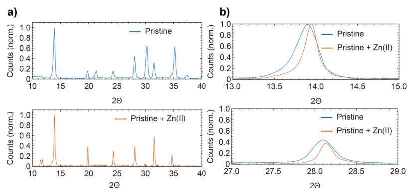
Figure 1. (a) XRD patterns of the pristine perovskite compared to the pristine containing Zn(II). (b) Magnification of the two highest diffraction peaks corresponding to (110) and (220) planes. The shift to higher 2\theta indicates the incorporation of Zn(II).
