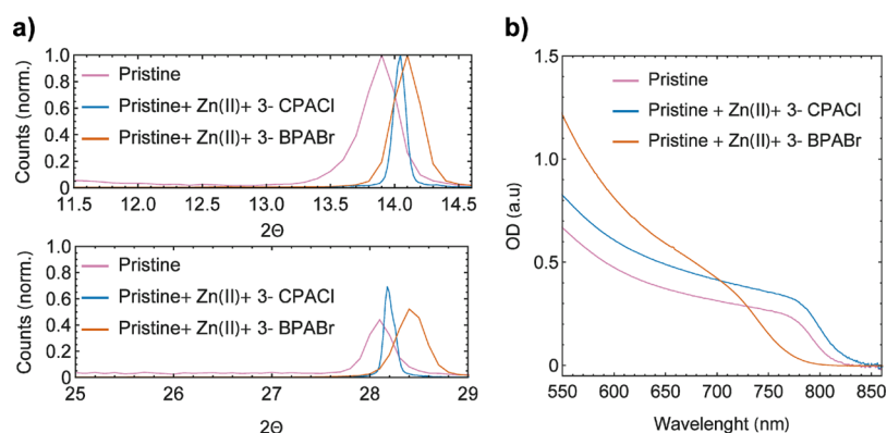
Figure 5. (a) XRD pattern magnification for the (100) and (200) of the pristine material, pristine containing Zn(II) and 3-CPACl, and the one containing Zn(II) and 3-BPABr. (b) UV-vis of the pristine material, the perovskite containing Zn(II) and treated with 3-BPABr and 3-CPACl.
