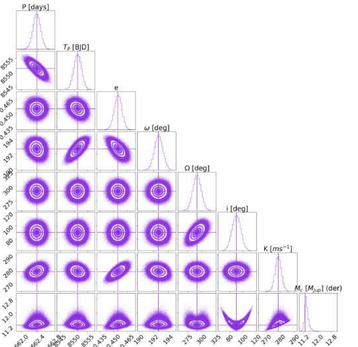
Fig. B.8. Posterior distributions of HD 141937 system over the full range of orbital inclinations.
