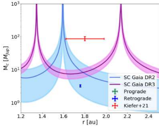
Fig. 5. Sensitivity curve for HD 5388 companion. The blue line is the sensitivity curve derived using GDR2 with its 1\sigma level of confidence. The red cross represents the value obtained by Kiefer et al. (2021) using GASTON. The green cross represents the prograde value, while the blue cross corresponds to the retrograde value we obtained using GDR3 in this work. Our results are compatible with the sensitivity curve.
