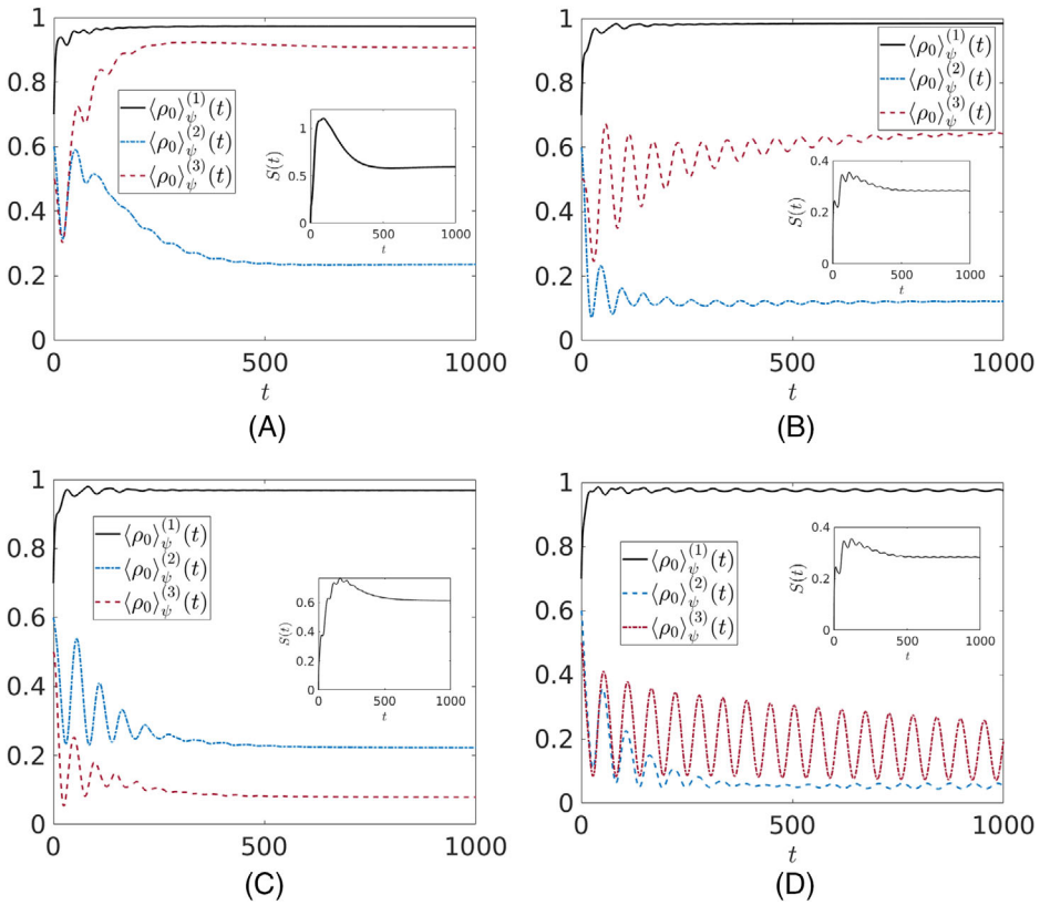
FIGURE 6 (A) The time evolution of the expected value \langle \rho_0 \rangle_\psi^{(1,2,3)}(t) for the three parties model with the add of a second Lindblad operator \kappa \hat{a}_2^\dagger . Nonzero parameters are: \kappa = 0.1 , \omega_1 = \omega_2 = \omega_3 = 0.1 , \lambda_1 = \lambda_2 = \lambda_3 = 0.025 , \gamma_1 = 1 , \tau_1 = 0.5 . Initial state is such that \langle \rho_0 \rangle_\psi^{(1)}(0) = 0.7 , \langle \rho_0 \rangle_\psi^{(2)}(0) = 0.6 , \langle \rho_0 \rangle_\psi^{(3)}(0) = 0.5 . In the inset the time evolution of the entropy S . (B) Same plots as in (A) with \gamma_2 = 1, \gamma_1 = 0 , and the same other parameters and initial conditions. (C) Same plots as in (A) with \gamma_3 = 1, \gamma_1 = 0 , and the same other parameters and initial conditions. (D) Same plots as in (A) with \gamma_4 = 1, \gamma_1 = 0 , and the same other parameters and initial conditions.
