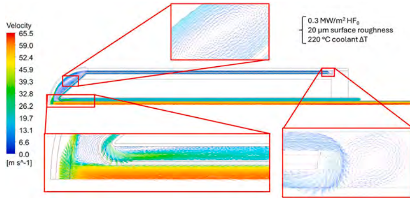
Fig. 6. Fluid velocity vector plot: details of vortices and fluid vein detachments.
