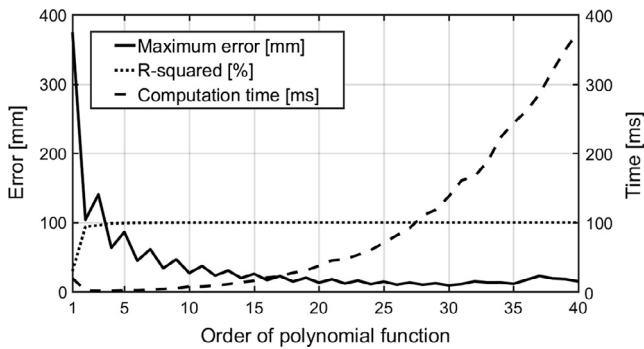
Fig. 2. Maximum error, R-squared parameter and computation time, plotted against the order of the fitting polynomial function.
