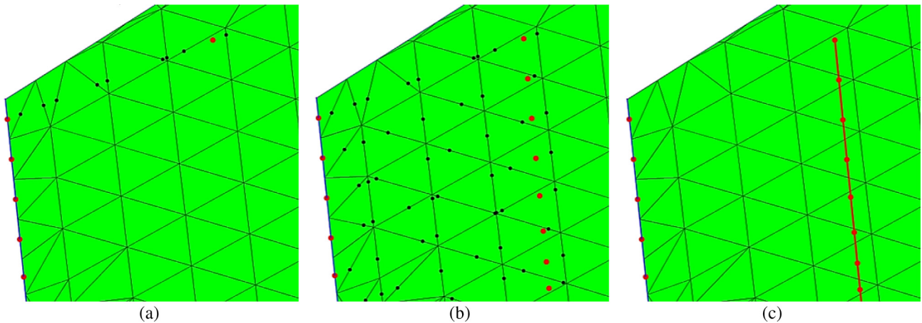
Fig. 6. Step-by-step process for the generation of a curve parallel to the reference edge.
