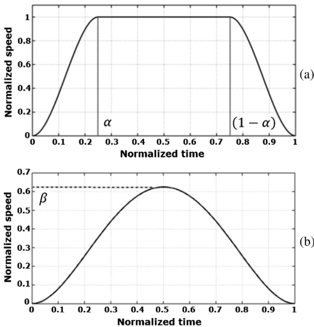
Fig. 12. Typical speed pattern for a long continuous curve (a) and a short one (b).
