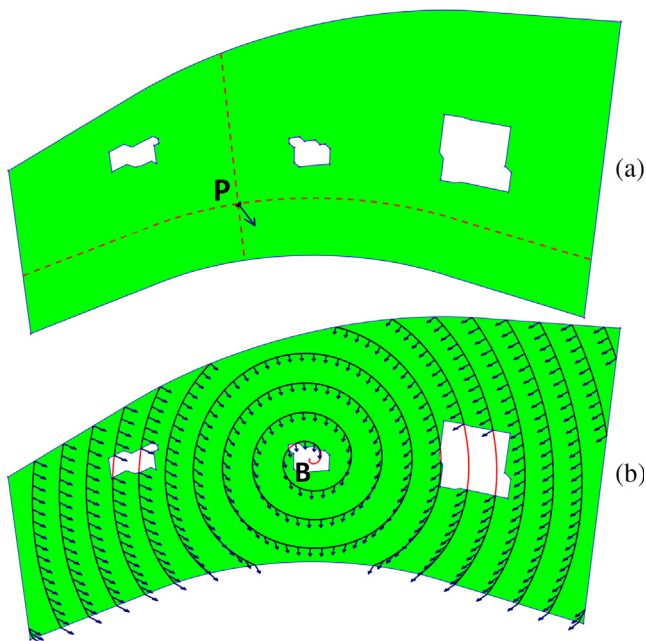
Fig. 9. Point at given distance from two edges (a) and spiral trajectory (b).
