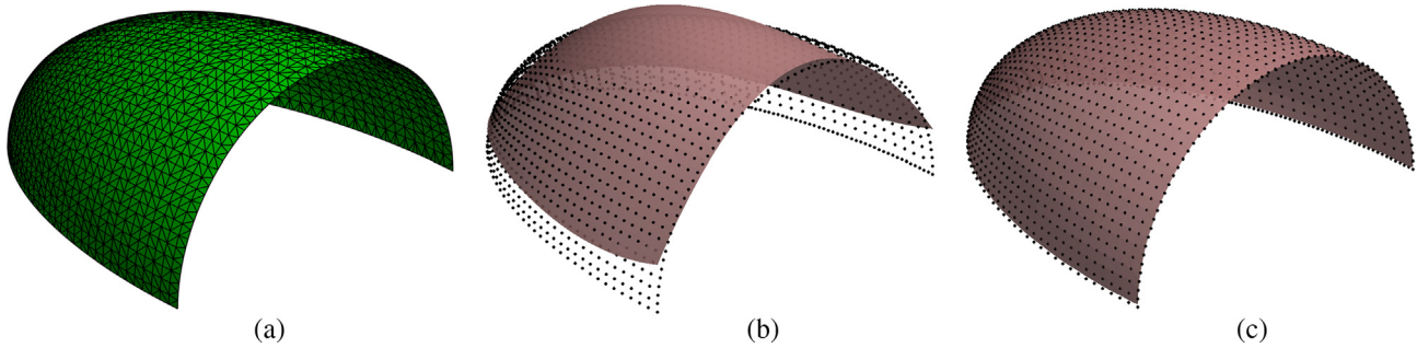
Fig. 1. Tessellated surface of one quarter of ellipsoid (a), approximation with 3rd order polynomial function (b) and with 30th order function (c).
