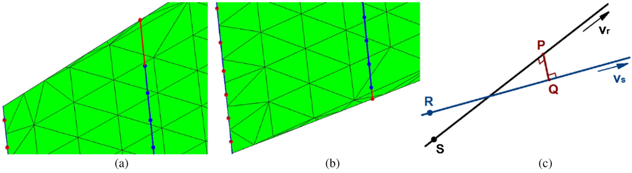
Fig. 7. Extension of trajectory to the surface boundary. First extremity (a) and second extremity (b). Minimum distance between two skew lines (c).
