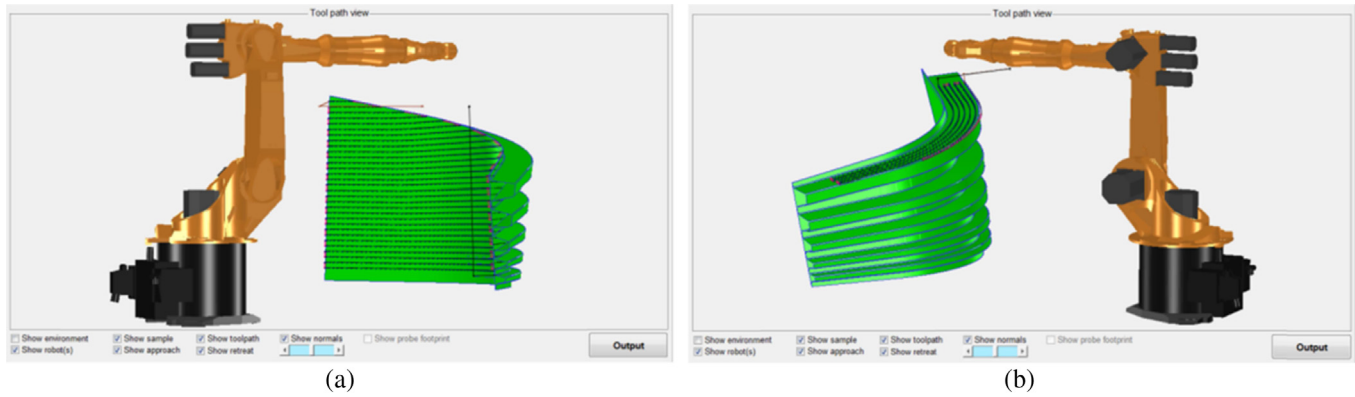
Fig. 13. Evaluation of generated tool-paths.
