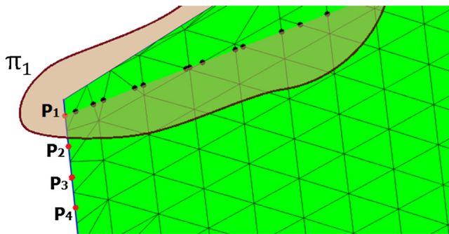
Fig. 5. Intersection points between mesh and plane for P_1 .
