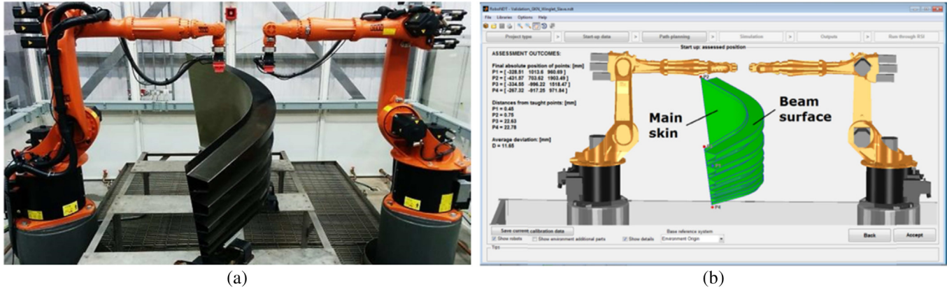
Fig. 10. Calculated position of the sample, waiting for the user to approve.
