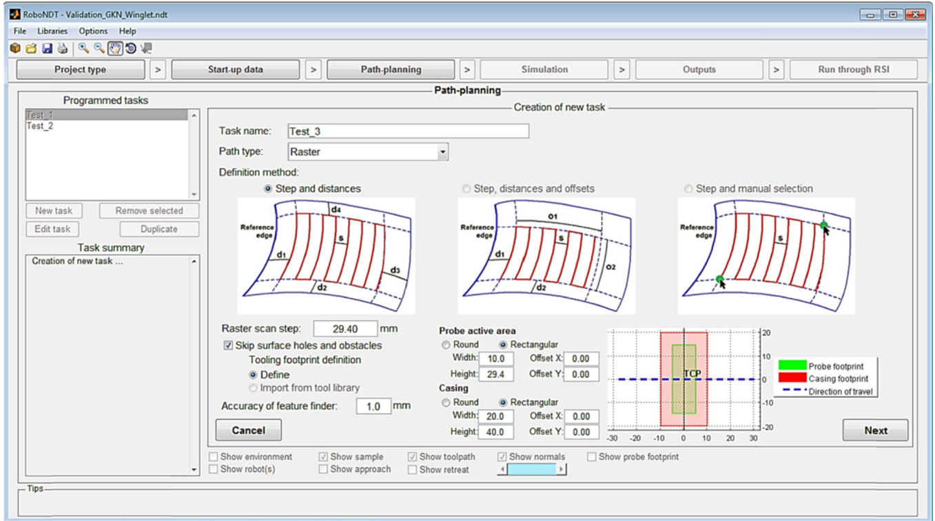
Fig. 11. RoboNDT path-planning GUI, developed to exploit the potentialities of the MFT method.
