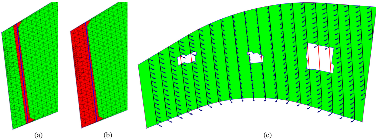
Fig. 8. Triangles crossed by the parallel curve (a), meshed region to be excluded (b) and completed iteration of algorithm (c), showing generated normals to the surface.
