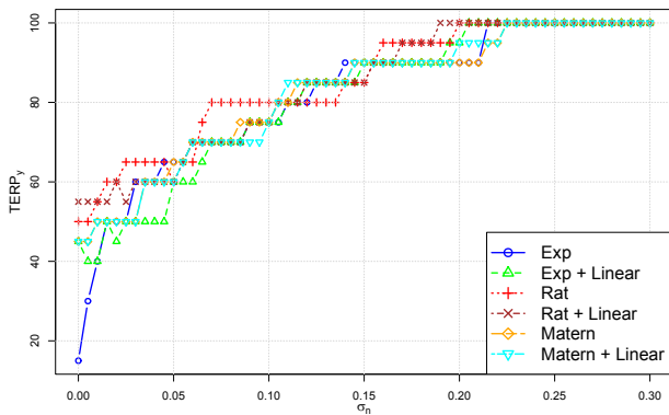
Figure 6: The amount of TERP for y coordinates versus versus Noise kernel parameter for EXP, Matern, Linear and some combination of these kernels.
