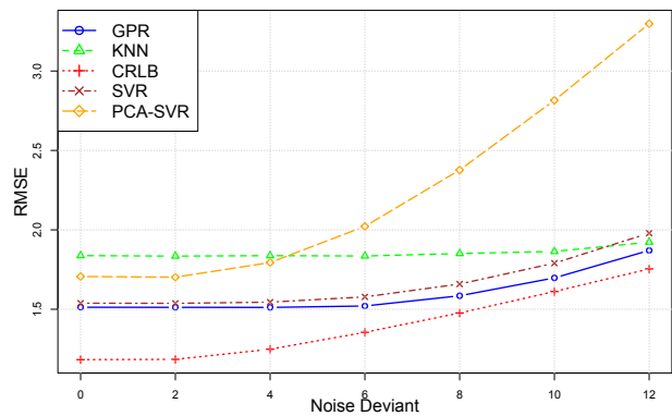
Figure 8: Localization error of proposed method (GPR) in compared with KNN, SVR, PCA-SVR and CRLB in terms of RMSE.
