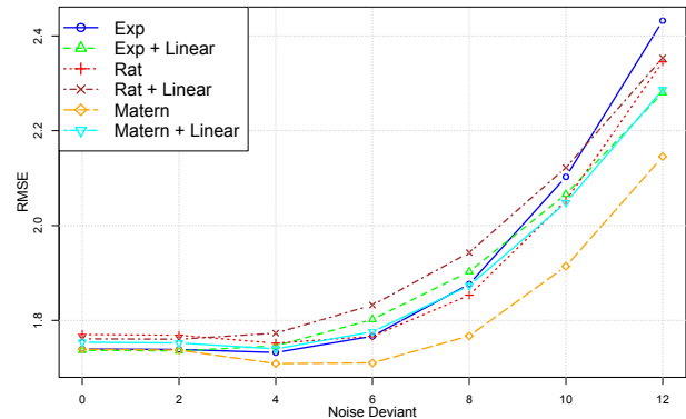
Figure 7: Positioning error of proposed method in terms of RMSE for different types of kernels.
