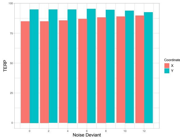
Figure 9: The amount of TERP versus the noise that shows the percentage of correctly estimated locations in 2\sigma confidence interval.
