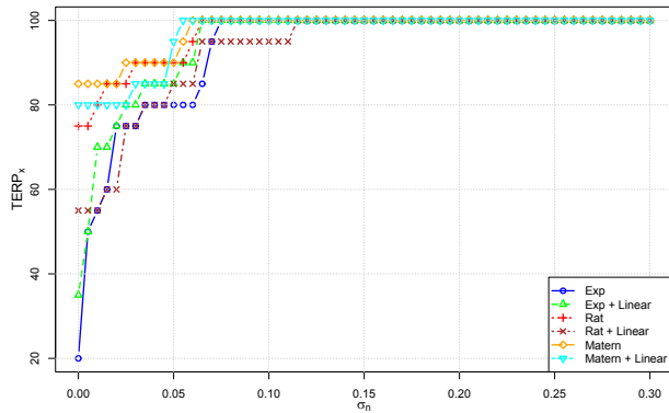
Figure 5: The amount of TERP for x coordinates versus Noise kernel parameter for EXP, Matern, Linear and some combinations of these kernels.
