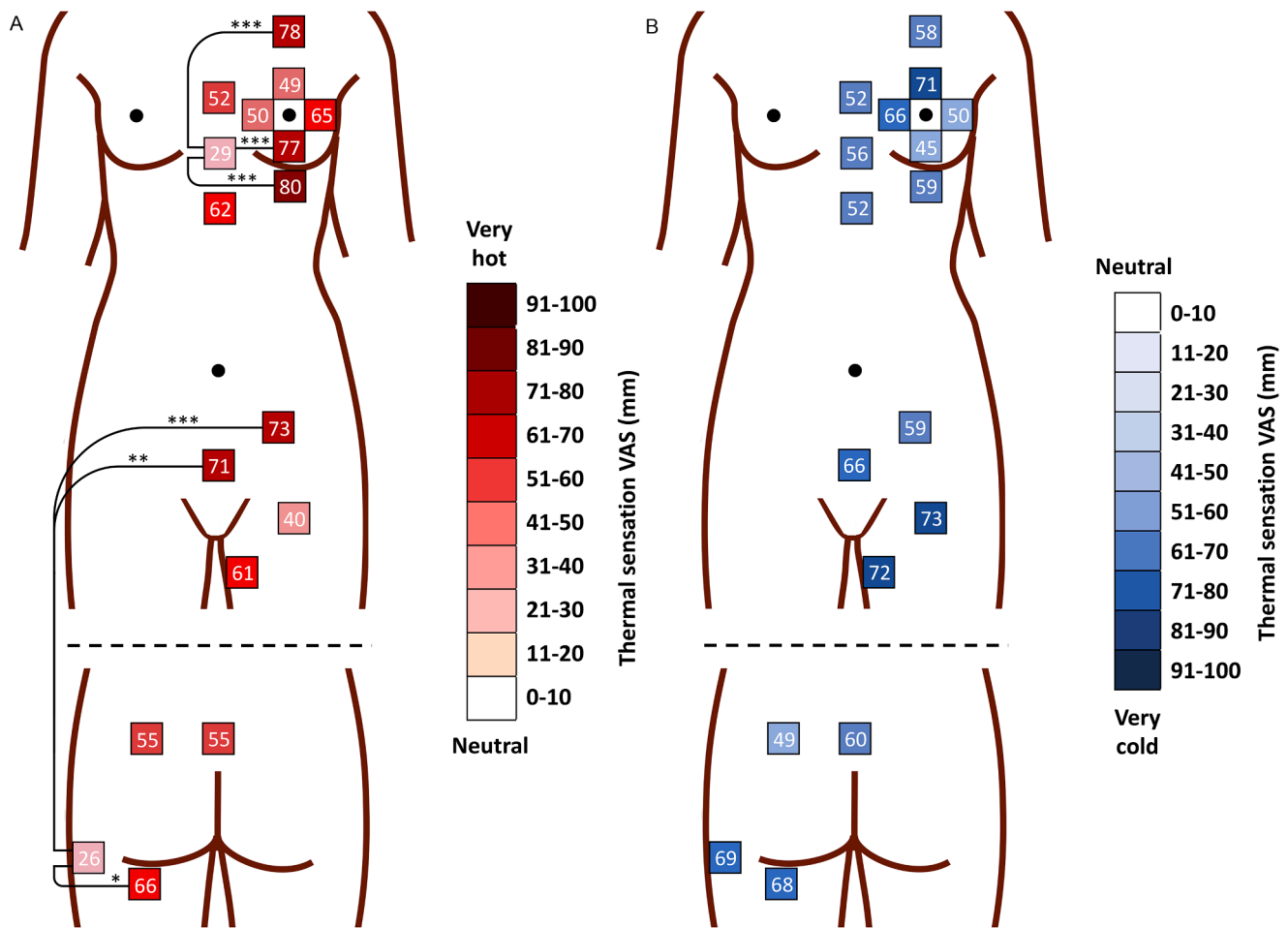
Fig. 3. Mean ( N = 12 ) warm (A) and cold (B) sensitivity for the 17 locations tested. Statistically significant multiple comparisons are picture (* p < 0.05 ; ** p < 0.01 ; *** p < 0.001 ). Statistical significance values for multiple location comparisons are listed in Electronic Supplementary Material.
