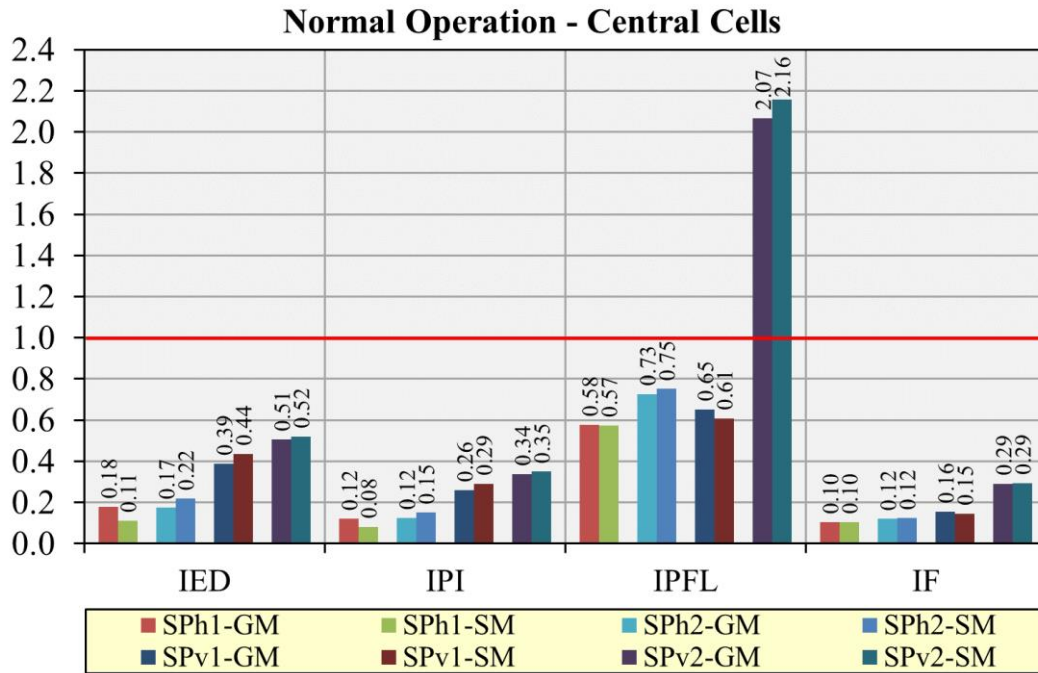
Figure 23 - RCC-MRx criteria evaluation within global model and CC sub-model in NO scenario.
