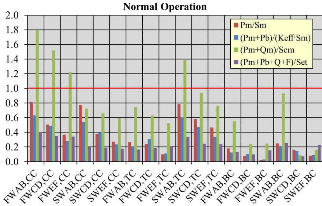
Figure 15 - RCC-MRx criteria verification in NO loading scenario within FW-SW.
