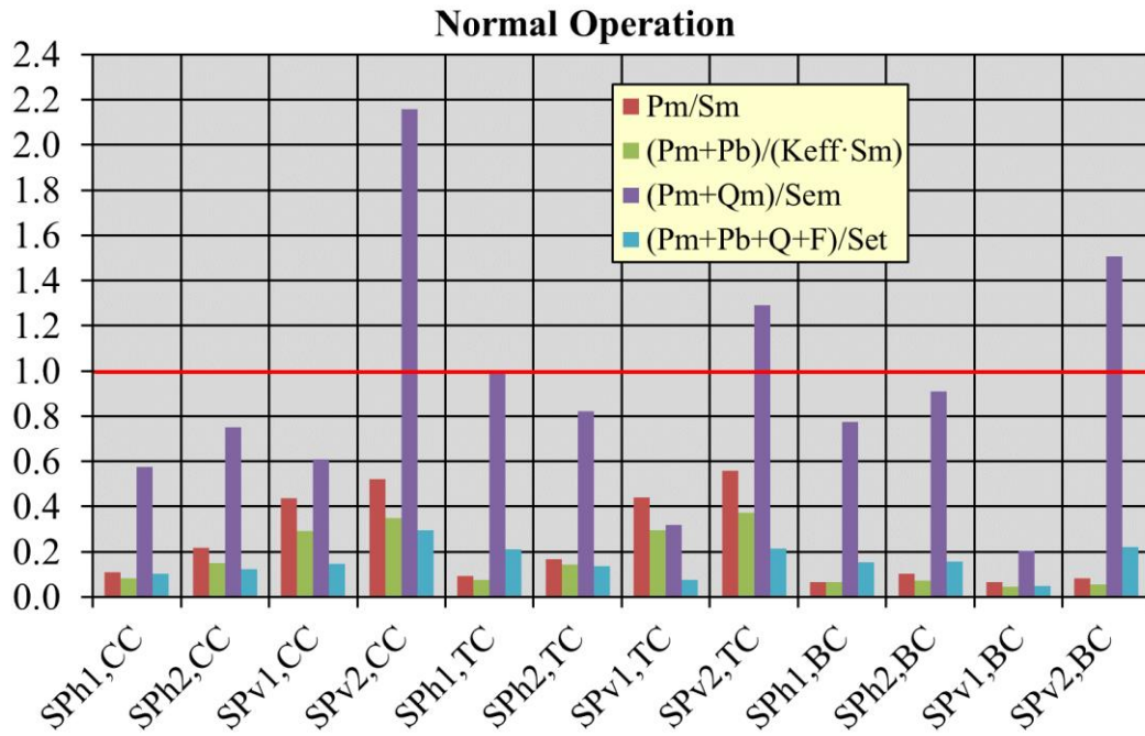
Figure 19 - RCC-MRx criteria verification in NO loading scenario within SPs.
