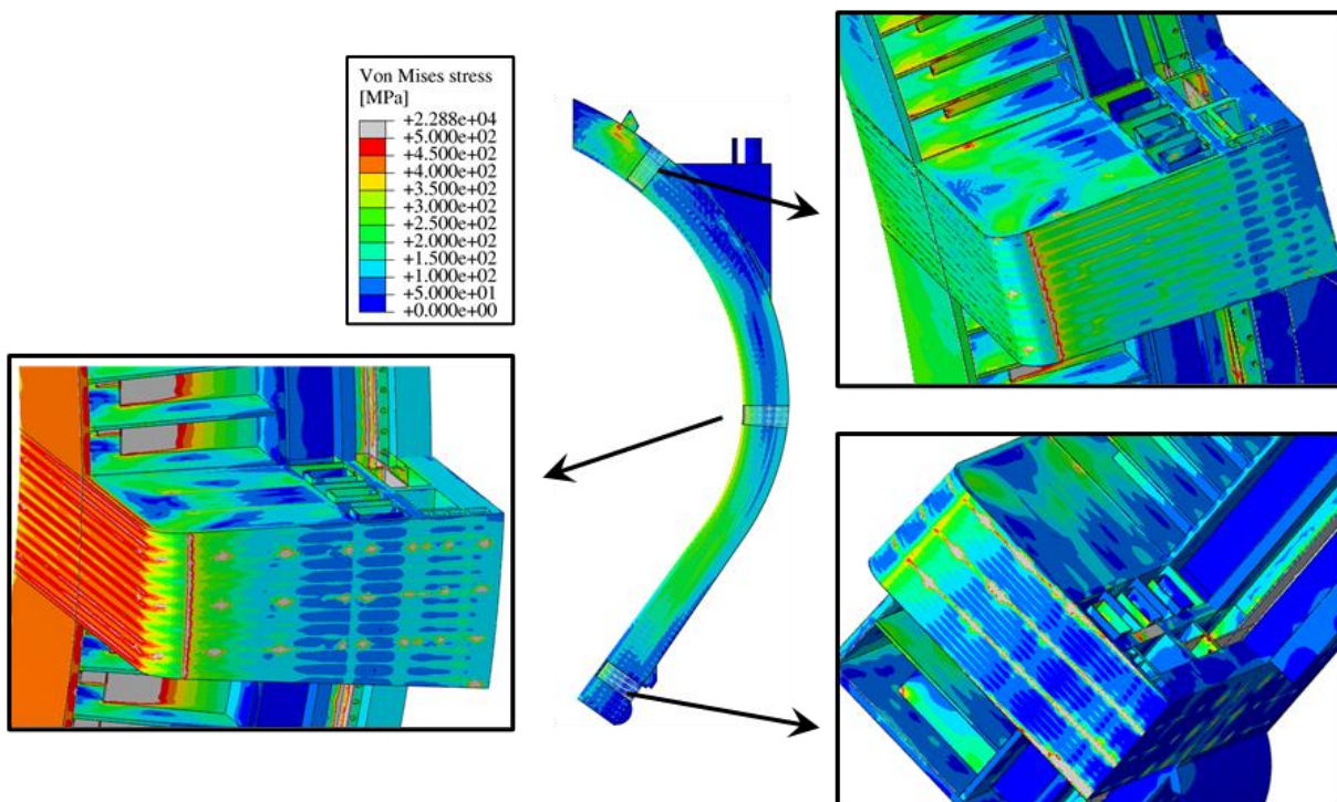
Figure 12 - Von Mises stress field within Top, Central and Bottom models in UVDE (t=11.585 s) superimposed to the global model Von Mises stress field.
