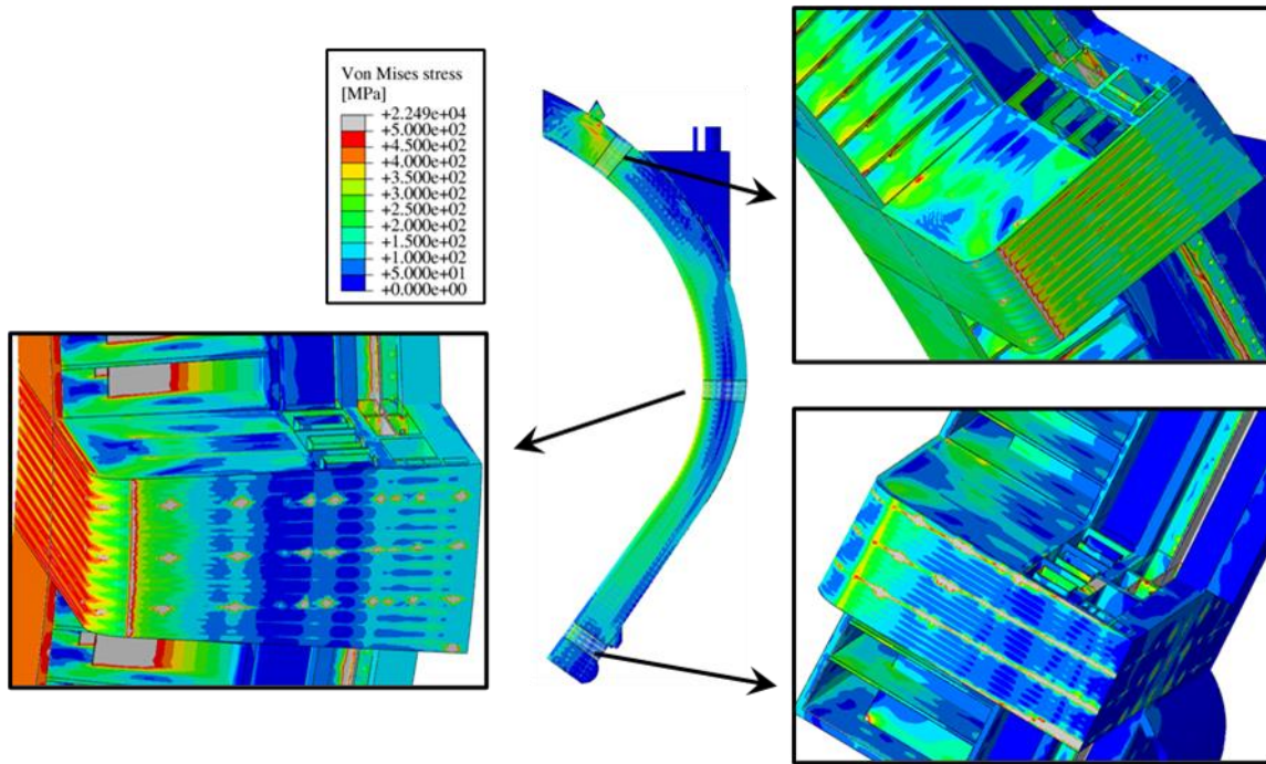
Figure 9 - Von Mises stress field within Top, Central and Bottom models in NO superimposed to the global model Von Mises stress field.
