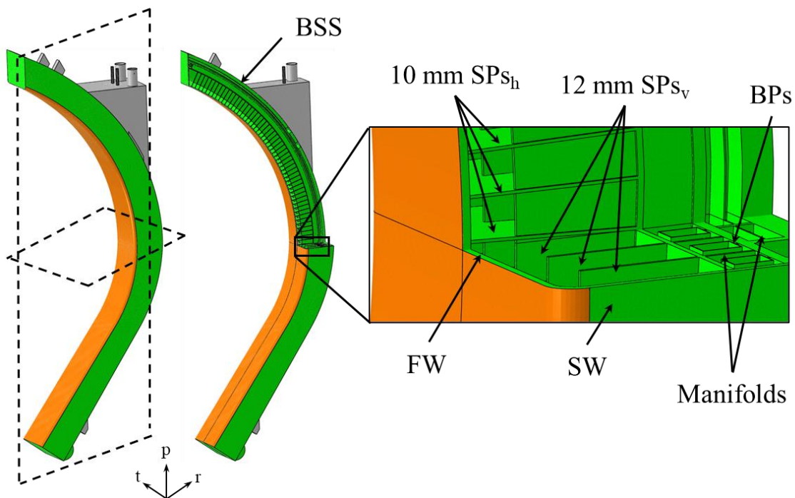
Figure 1 - WCLL COB segment architecture.
