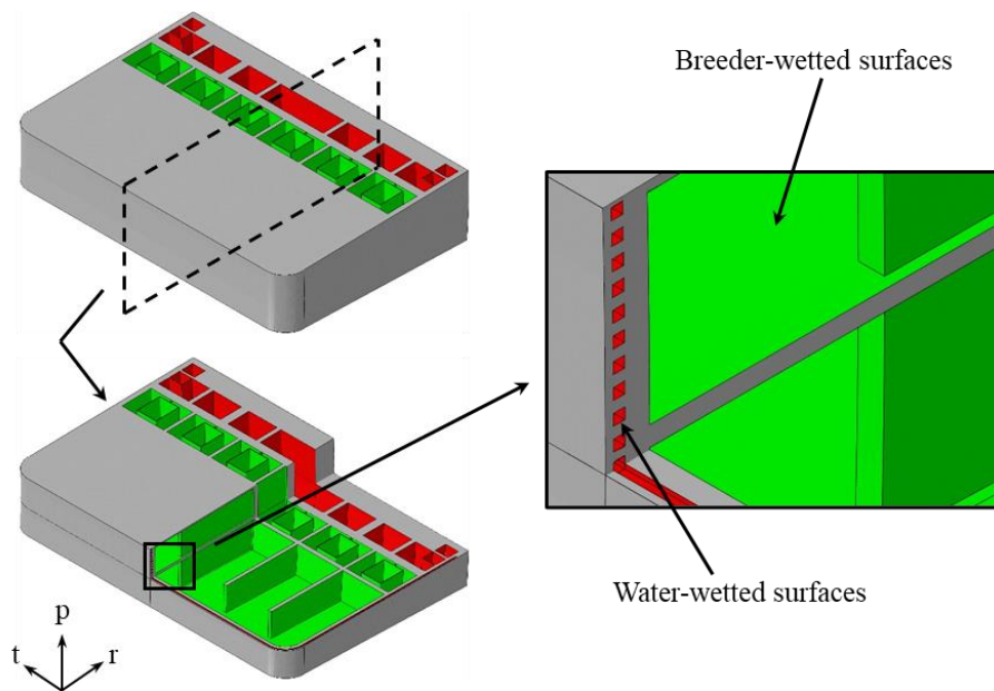
Figure 6 - Water and breeder wetted surfaces.
