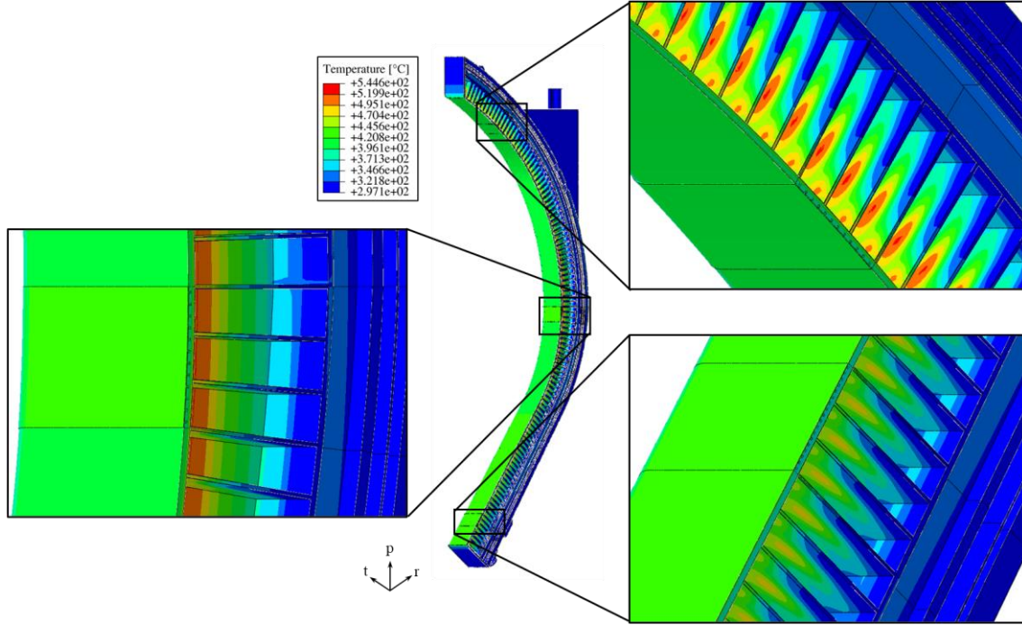
Figure 5 - Temperature field onto Top, Central and Bottom models superimposed to the global model.
