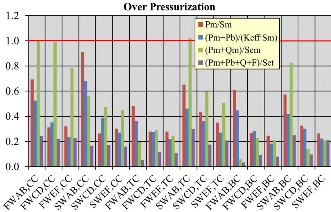
Figure 16 - RCC-MRx criteria verification in OP loading scenario within FW-SW.
