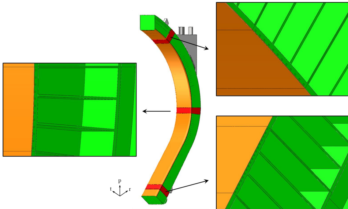
Figure 2 - Location of Top, Central and Bottom cells in the COB segment.
