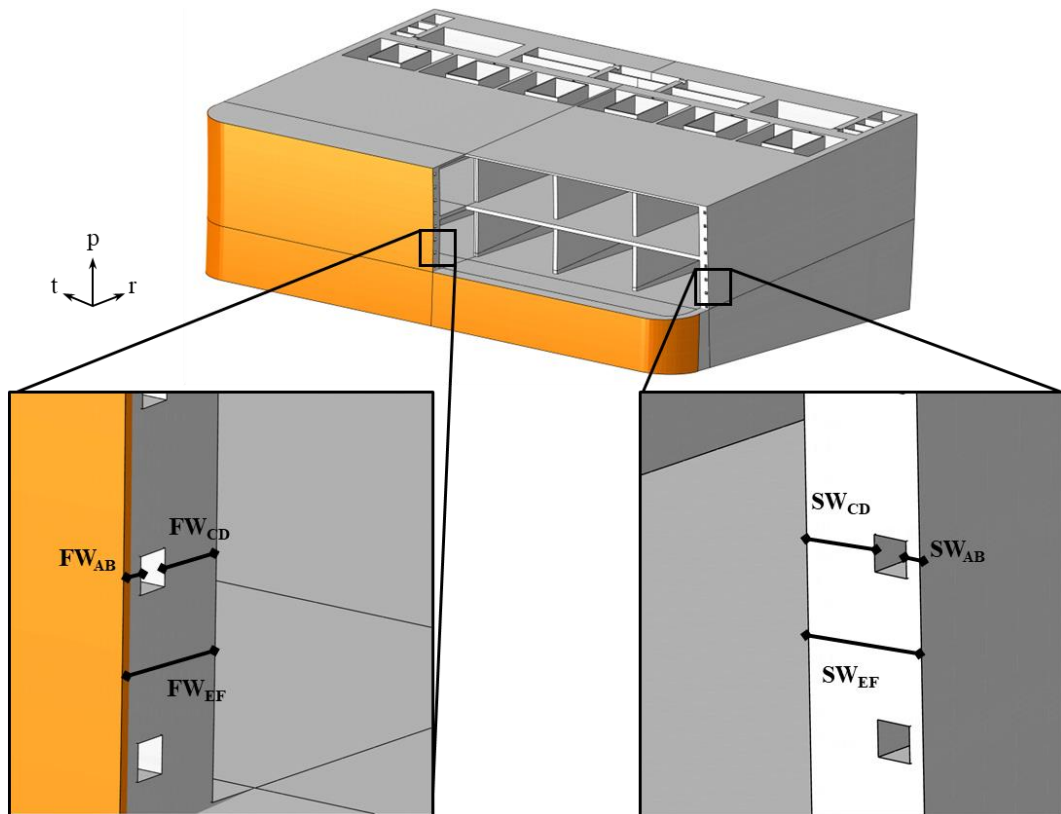
Figure 13 - Paths selected within FW-SW region in CC model.
