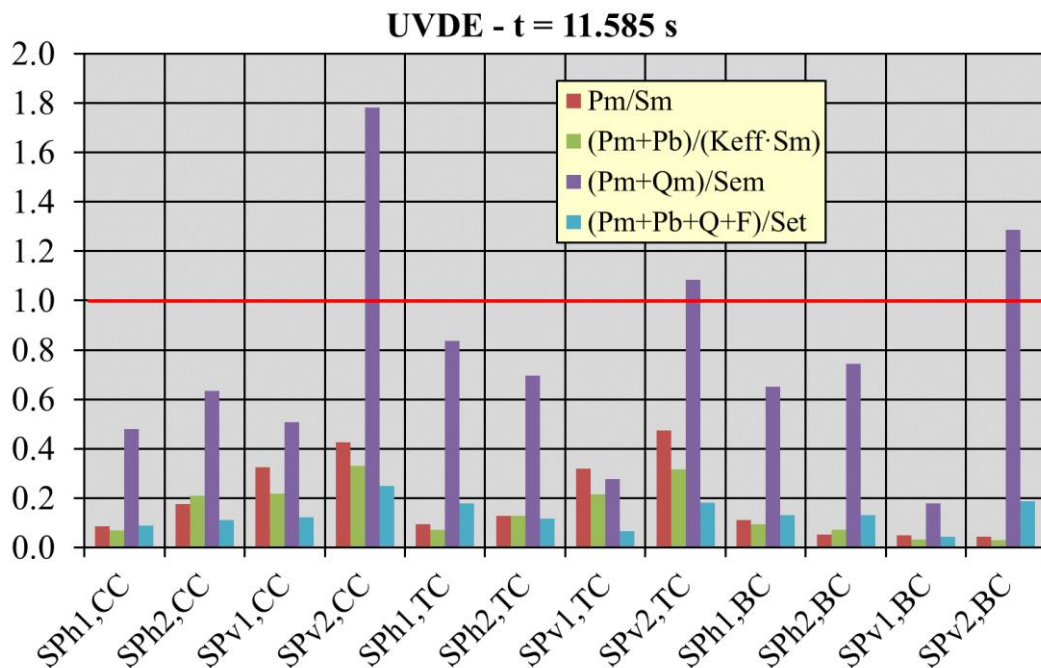
Figure 22 - RCC-MRx criteria verification in UVDE (t=11.585 s) loading scenario within SPs
