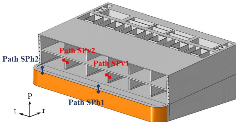
Figure 13 - Paths selected within FW-SW region in CC model.
