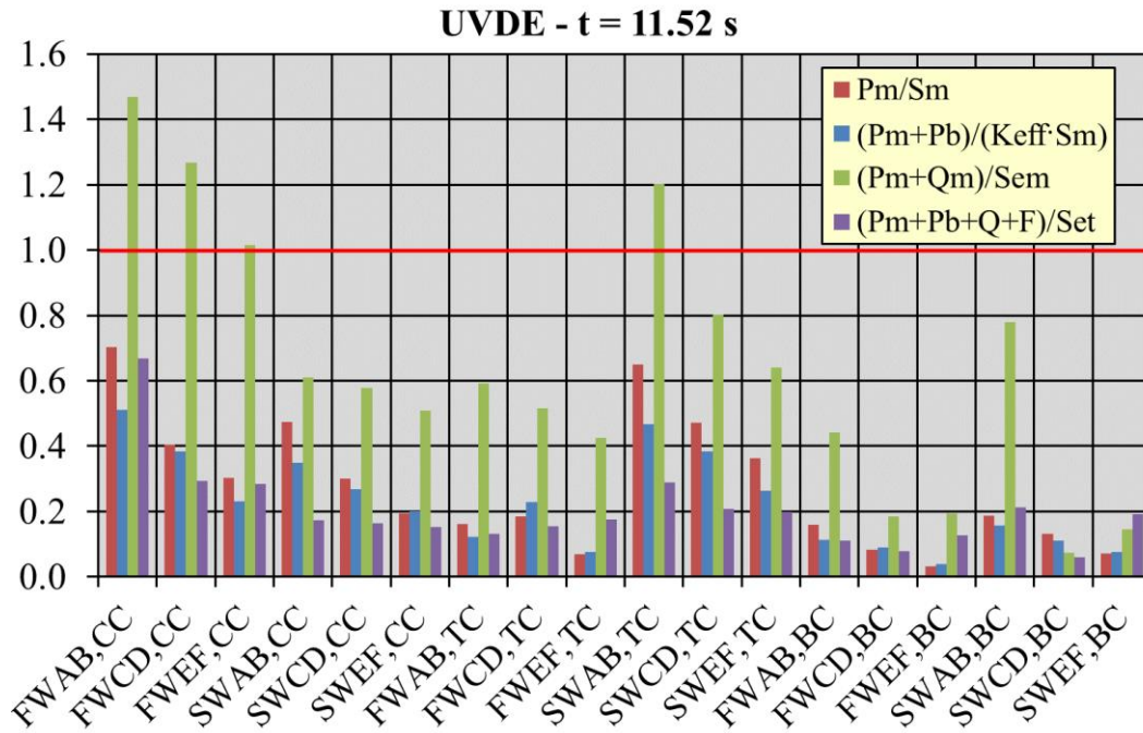
Figure 17 - RCC-MRx criteria verification in UVDE (t=11.52 s) loading scenario within FW-SW.
