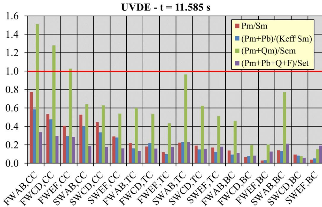
Figure 18 - RCC-MRx criteria verification in UVDE (t=11.585 s) loading scenario within FW-SW.
