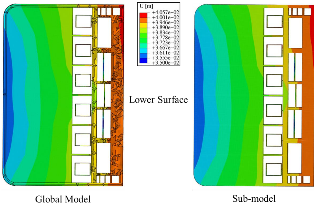
Figure 7 - Displacement field in global model and sub-model applied in NO scenario to the lower boundary of the central cells sub-model.
