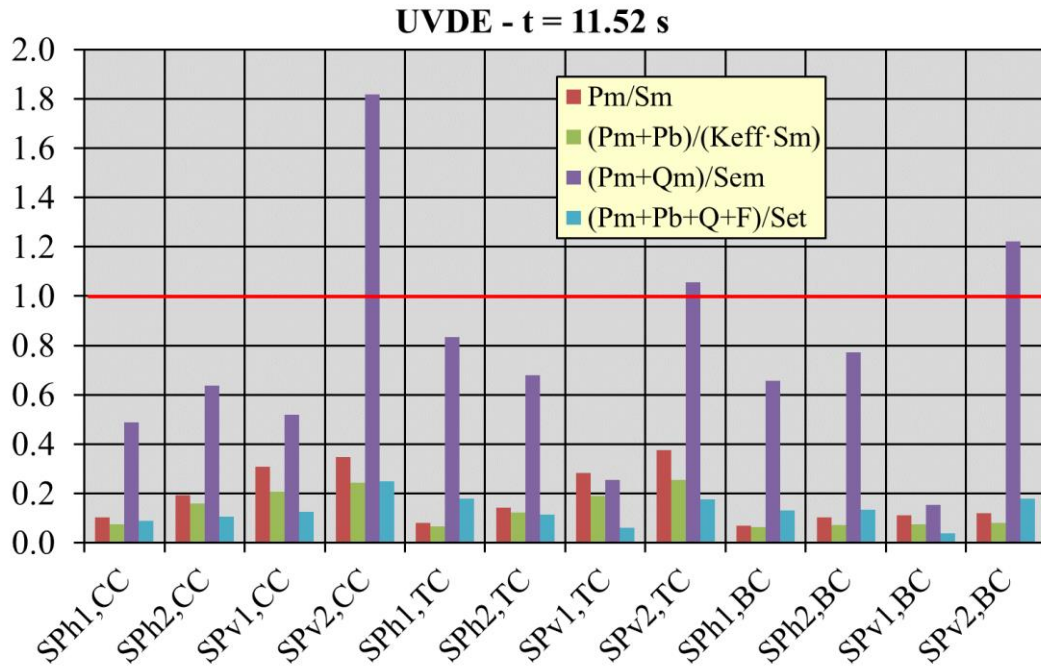
Figure 21 - RCC-MRx criteria verification in UVDE (t=11.52 s) loading scenario within SPs.
