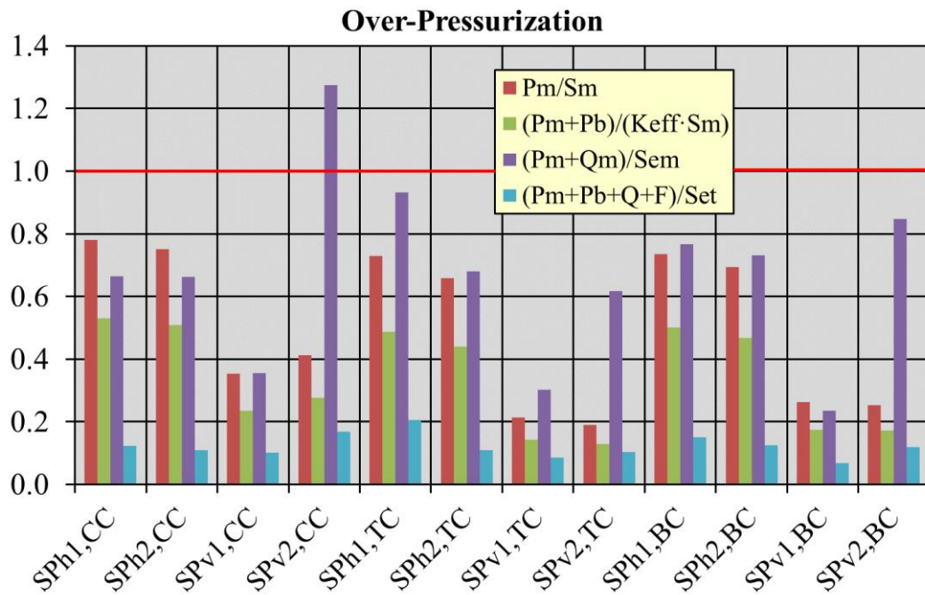
Figure 20 - RCC-MRx criteria verification in OP loading scenario within SPs.
