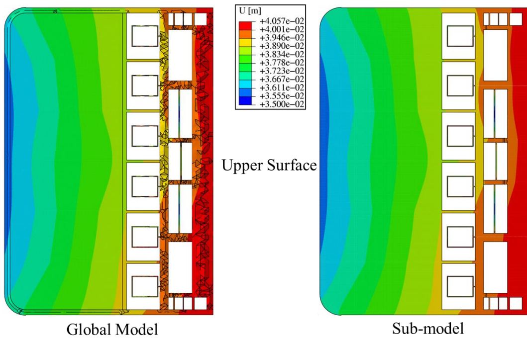
Figure 8 - Displacement field in global model and sub-model applied in NO scenario to the upper boundary of the central cells sub-model.
