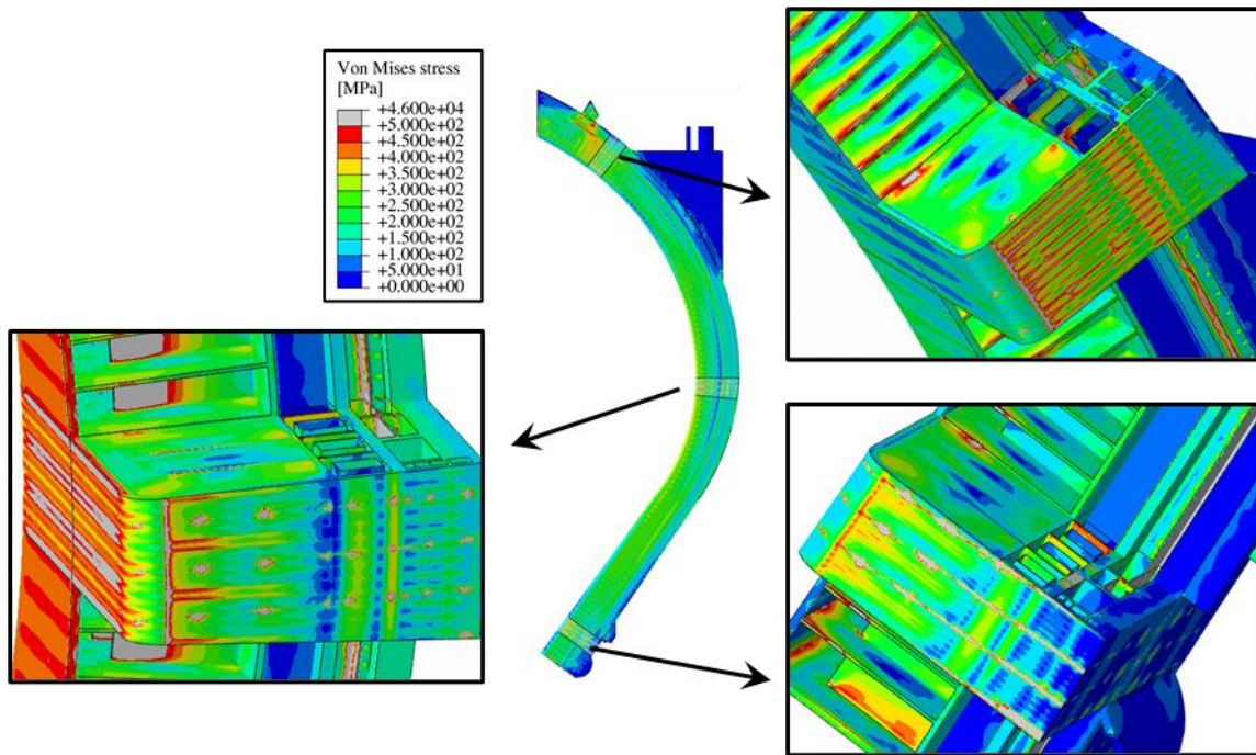
Figure 11 - Von Mises stress field within Top, Central and Bottom models in UVDE (t=11.52 s) superimposed to the global model Von Mises stress field.
