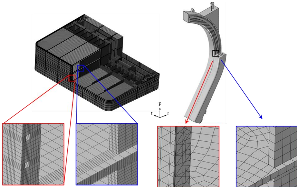
Figure 4 - Mesh of the CC sub-model vs mesh of the global model in the COB segment.
