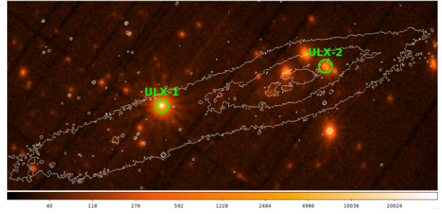
Figure 1. XMM-Newton stacked image of NGC 55. Circles with 20 arcsec radii are drawn around the ULXs along with surface brightness contours from the filter-RG610 DSS image. The colour bar shows the number of counts.
