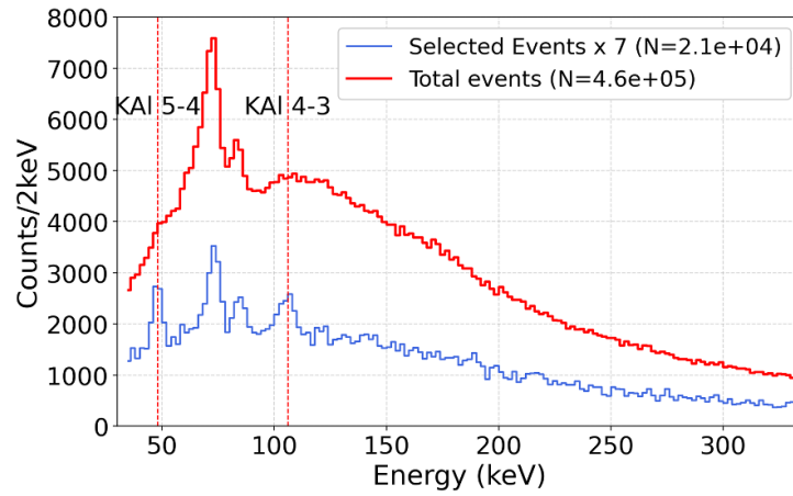
Figure 11. Histogram of the raw spectrum (red), compared to the one after the optimized selections with counts multiplied by a factor 7 (blue), with the kaonic aluminum transitions highlighted in red.
