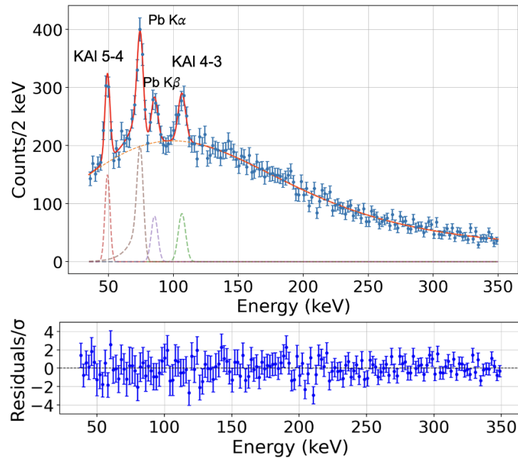
Figure 12. Fit to the data after the optimized selection (up). The errors of the number of counts reported are the statistical errors ( 1/\sqrt{\text{counts}} ). The plot of residuals for each bin normalized at their standard deviation ( \sigma ) is also reported (down).
