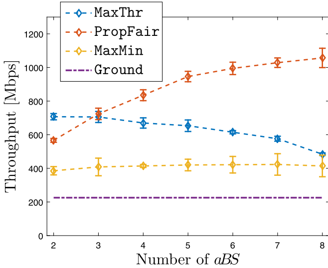
Fig. 13. Throughput of stadium users for \alpha \in \{0, 1, \infty\} . G = 10 , U = 1000 . Scenario: Stadium with U_d = 600 .
