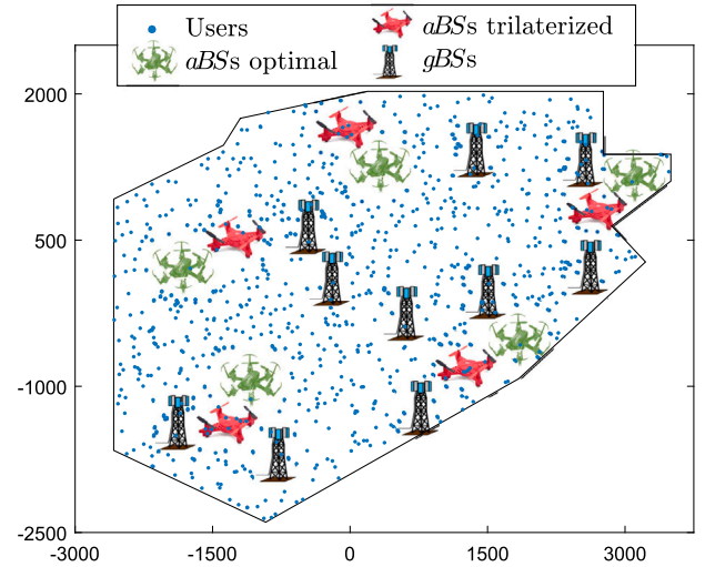
Fig. 10. Robustness validation for \alpha = 1 . aBSs placement error. G = 10 , A = 5 , U = 1000 . Scenario: PPP.
