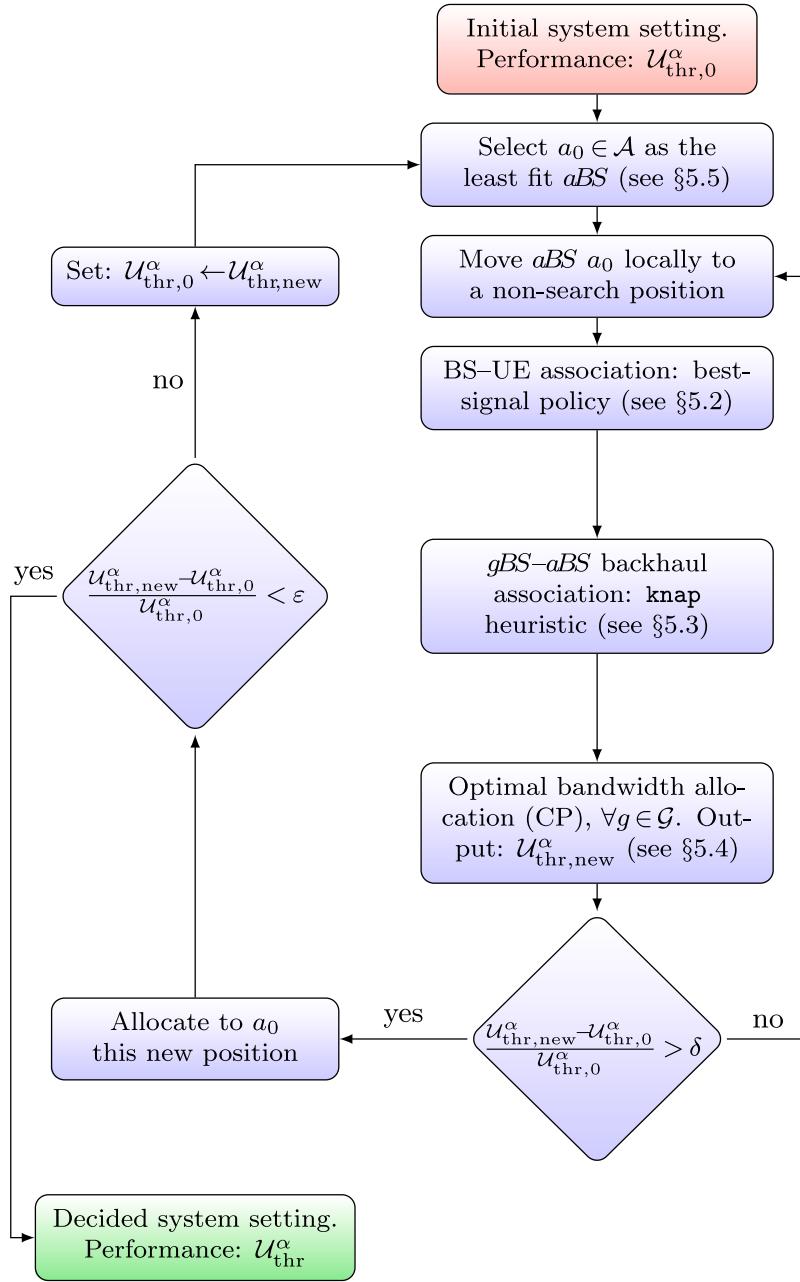
Fig. 4. Flow diagram of PADD operation.
