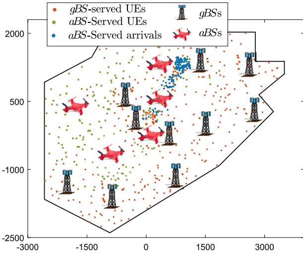
Fig. 14. Network state at t = 25 min. G = 10 , A = 5 , U = 640 . Scenario: PropFair, Event.
