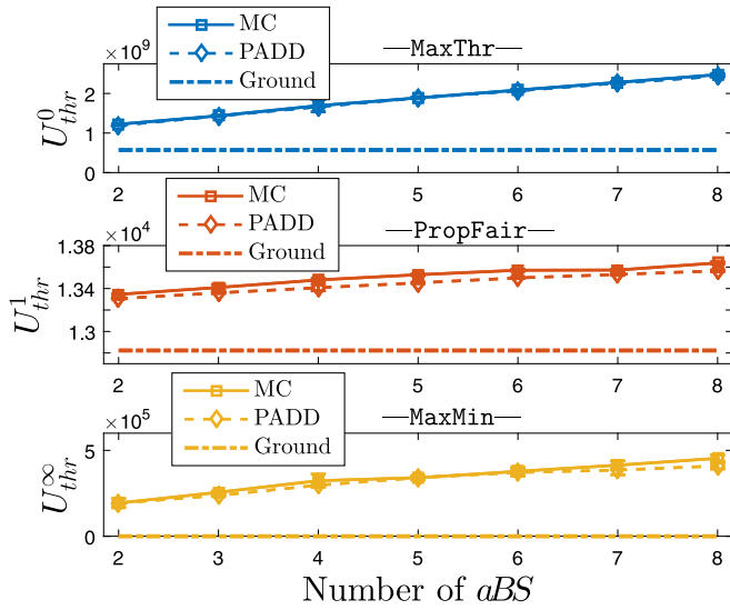
Fig. 8. Utility validation for \alpha \in \{0, 1, \infty\} . G = 10 , U = 1000 . Scenario: PPP.
