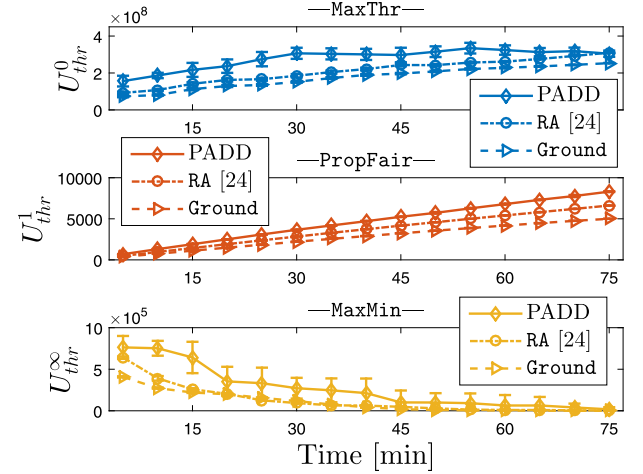
Fig. 17. Attendance utility for \alpha \in \{0, 1, \infty\} . G = 10 , A = 5 , U = [400, \dots, 1000] . Scenario: Event.
