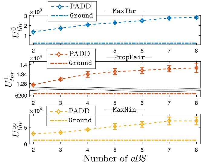
Fig. 11. Utility of all users for \alpha \in \{0, 1, \infty\} . G = 10 , U = 1000 . Scenario: Stadium with U_d = 600 .
