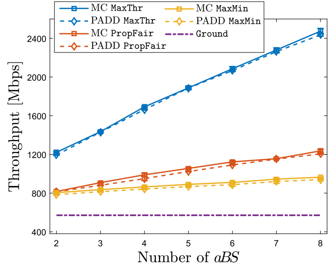
Fig. 9. Network capacity validation for \alpha \in \{0, 1, \infty\} . G = 10 , U = 1000 . Scenario: PPP.
