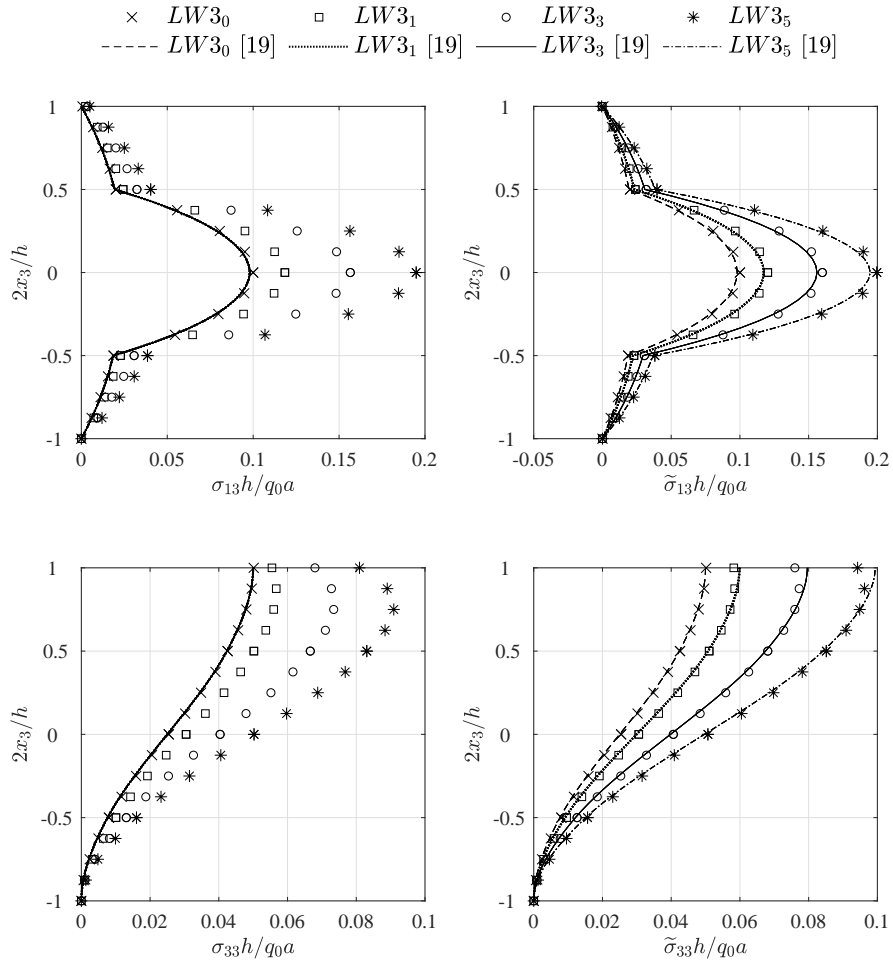
Figure 4: Through-the-thickness distribution of out of plane stress components at the point of in-plane coordinates (a/4, a/4) . Results for the 8 \times 8 mesh of 9-node isoparametric elements.
