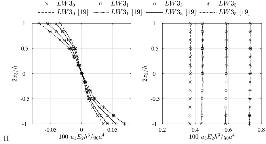
Figure 3: Through-the-thickness distribution of displacement components at the point of in-plane coordinates (a/4, a/4) . Results for the 8 \times 8 mesh of 16-node isoparametric elements.
