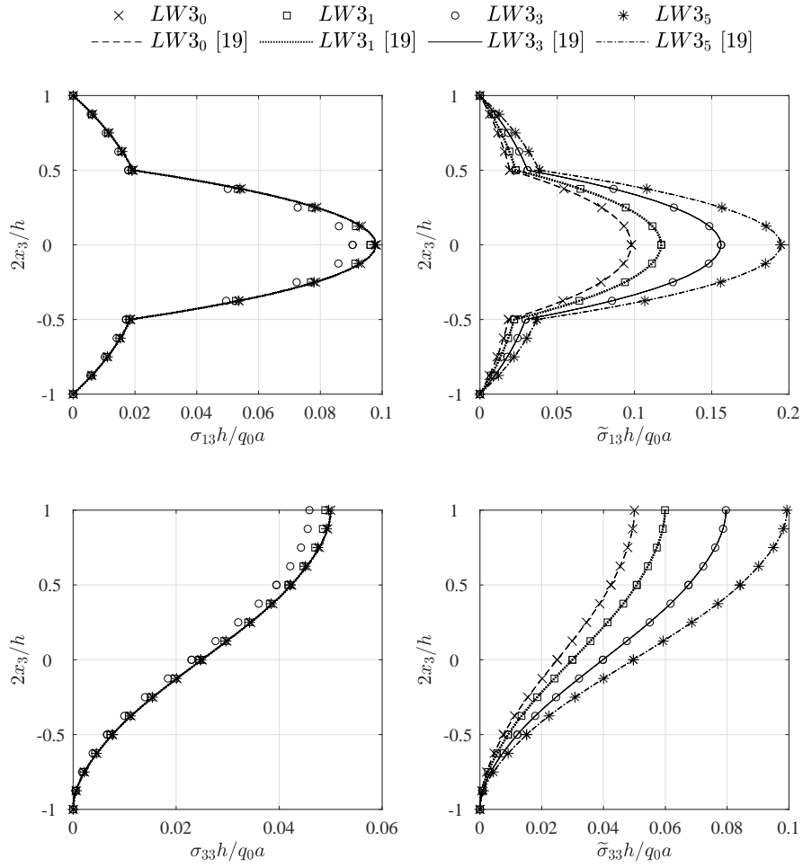
Figure 5: Through-the-thickness distribution of out of plane stress components at the point of in-plane coordinates (a/4, a/4) . Results for the 8 \times 8 mesh of 16-node isoparametric elements.
