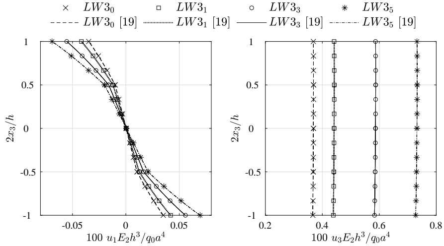
Figure 2: Through-the-thickness distribution of displacement components at the point of in-plane coordinates (a/4, a/4) . Results for the 8 \times 8 mesh of 9-node isoparametric elements.
