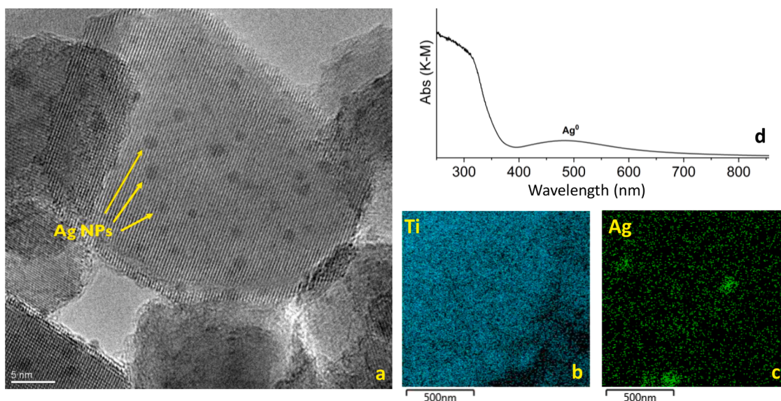
Fig. 2. a: HR-TEM image of the TiO 2 photocatalyst recovered after 180 min of UV-A irradiation in the presence of AgNO 3 10 mM and (R)-limonene 2 mM in acetonitrile. Silver nanoparticles (Ag NPs) are highlighted with yellow arrows; b: EDX map of titanium atoms (light blue points); c: EDX map of silver atoms (green points); d: UV-vis diffuse reflectance spectrum (DRS) of the same sample.
