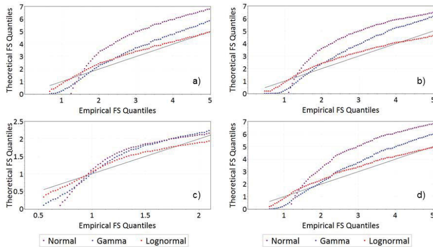
Fig. 2. Empirical FS quantiles (numerically derived) vs theoretical FS quantiles of Lognormal (red), Gamma (blue), and Normal (purple) distributions for (a) clay, (b) clay loam, (c) sandy loam, and (d) silty clay. The used values of slope, depth of failure surface and volumetric water content are equal to 40^\circ , 1000 mm and 0.3 \text{ mm}^3/\text{mm}^3 respectively, while the used values of statistical parameters are reported in Table 1.
