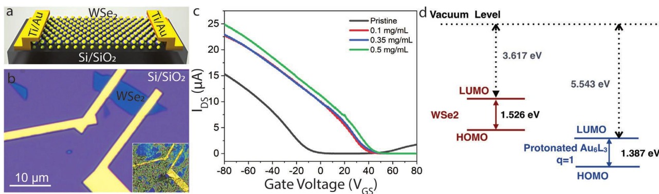
Figure 5. a) The schematic diagram and b) optical microscope image of the back gated WSe 2 field effect transistor. Inset: optical micrograph of WSe 2 device after deposition of GNCs. c) Transfer plots ( I_{DS} - V_{GS} ) obtained from the multilayer WSe 2 device before and after deposition of different concentration of GNCs at V_{SD} = 0.5 V. d) Theoretical calculations for the HOMO-LUMO states of [\text{Au}(\text{I})_6(\text{TRZ})_3]^+ and multilayer WSe 2 .
