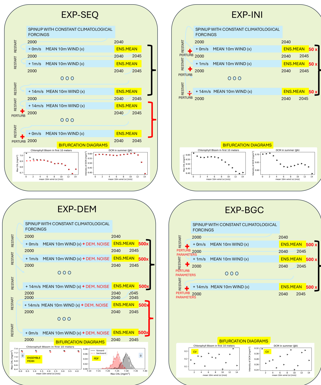
Figure 3. Protocols of the simulation experiments EXP-SEQ, EXP-INI, EXP-DEM, and EXP-BGC. The experiments methodology is described in Sect. 2.4. For each EXP we considered the effects of the perturbation of the 6 environmental forcings, listed in Table 1, over all the target indicators, listed in Table 2. Here the forcing 10 m wind ( x ) is taken as an example.
