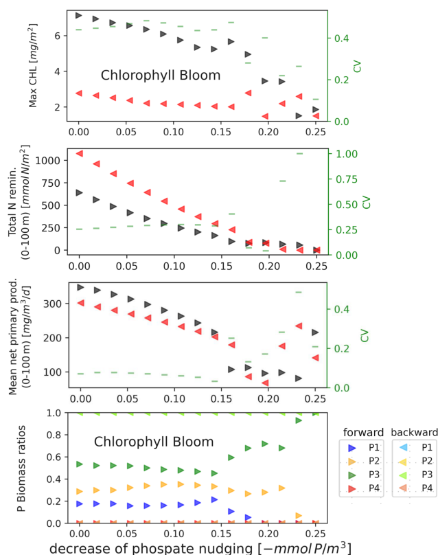
Figure 5. EXP-SEQ setup: Bifurcation diagrams showing the hysteretic response of the model's dynamic regimes associated to seasonal properties (top row), cycling (second row), annual production (third row) and community composition (bottom row) to phosphate nudging. The mean magnitude of the environmental forcings ( x axis) goes from its original value (left) to extreme values (right). The panels show the hysteresis, the forward path (black), from original to extreme environmental condition, and the backward path (red), from extreme to original environmental condition, follow different trajectories. The forward path, from original values to extreme values, is showed in darker colours. For community composition (bottom row) the forward path, from original values to extreme values, is showed in darker colours and the backward path, from extreme values to original values, is showed in lighter colours. Different colours indicates different phytoplankton functional types. In the backward simulations only P3 (in green) is present. The hysteresis has been quantified with CV > 0.1 , shown in green. The methodology is presented in Sect. 2.4.1.
