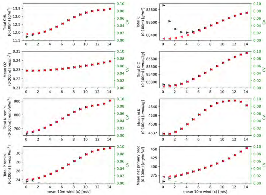
Fig. S2. Bifurcation diagrams under the variation of wind forcing in the EXP-SEQ experimental setup for the dynamic regimes associate with annual production and recycling. The black triangles stand for the simulations which follow the x-axis values with time (forward, from original to extreme environmental condition), the red triangle the simulations which go backwards (from extreme to original environmental conditions). The reversibility has been quantified with CV < 0.1 , shown in green.
