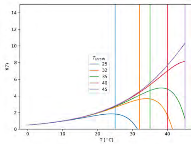
Fig. S10. Plot of the regulation function of temperature on metabolic rates (Eq. (S4)). The value of the threshold temperature T_{thresh} set the flex of the function.
