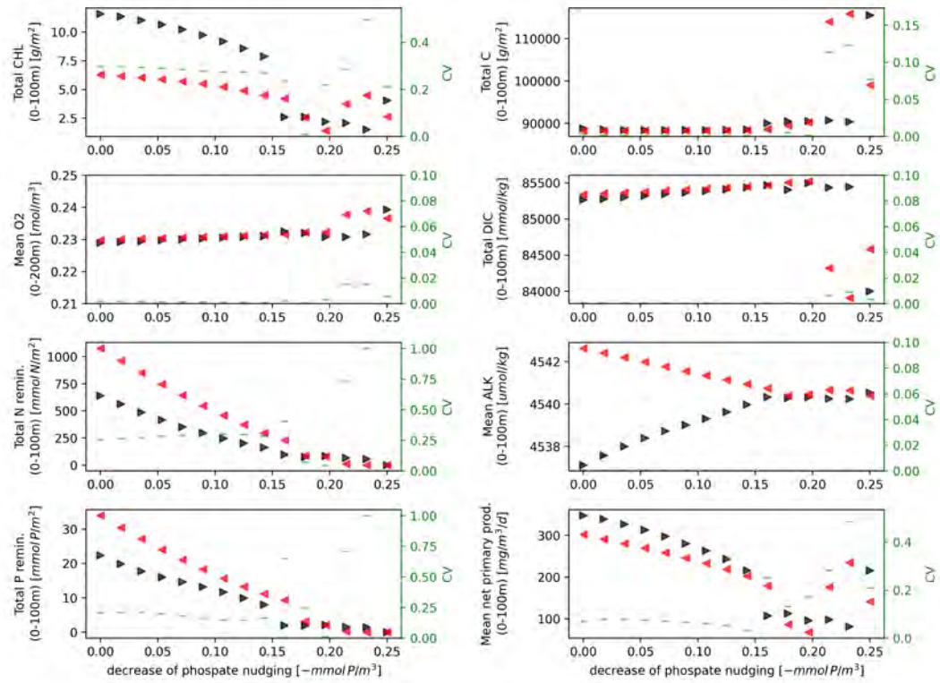
Fig. S6. Bifurcation diagrams under the variation of phosphate nudging forcing in the EXP-SEQ experimental setup for the dynamic regimes associate with annual production and recycling. The black triangles stand for the simulations which follow the x-axis values with time (forward, from original to extreme environmental condition), the red triangle the simulations which go backwards (from extreme to original environmental conditions). The hysteresis has been quantified with CV > 0.1 , shown in green.
