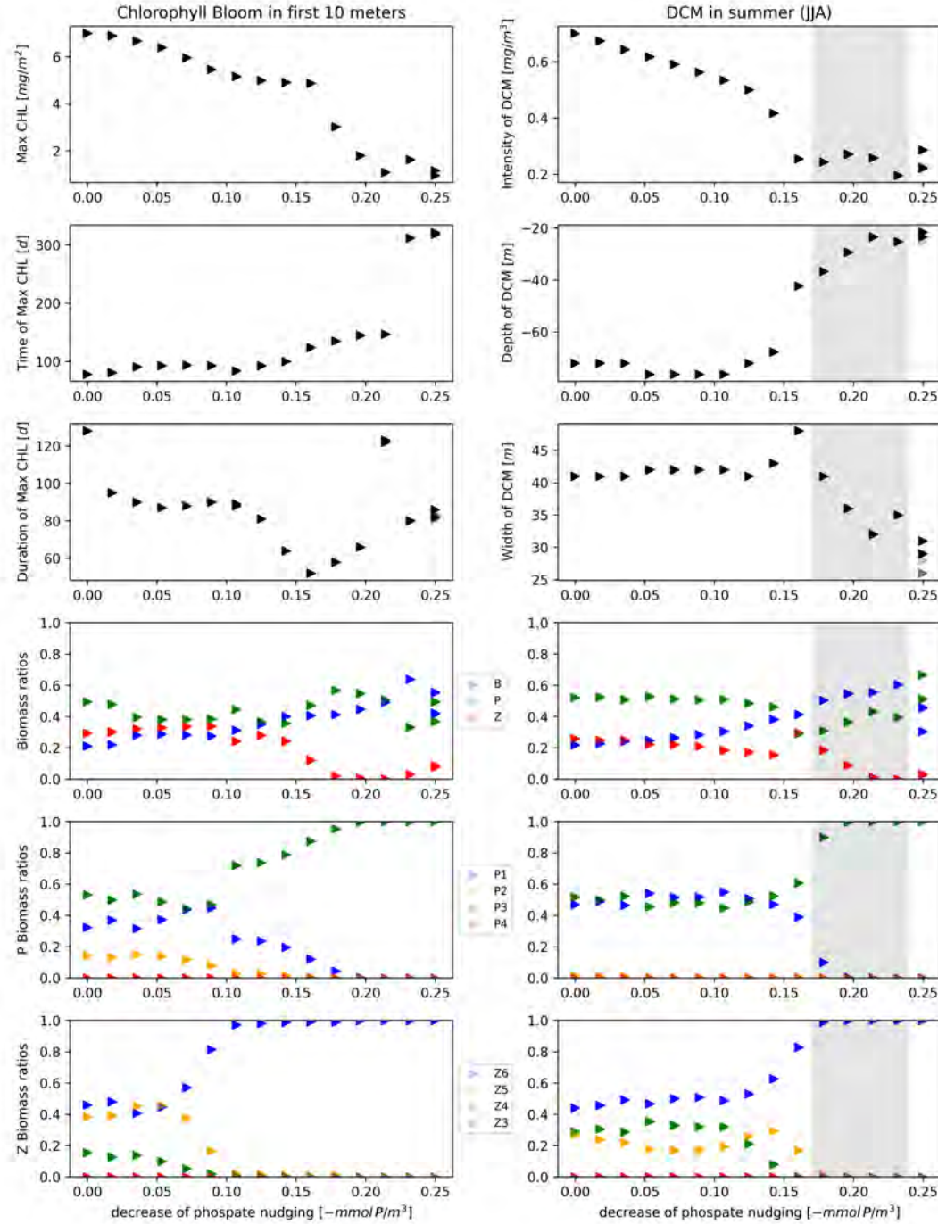
Fig. S9. Bifurcation diagrams for the properties of Chlorophyll bloom (left panels) and DCM (right panels) under the decrease of phosphate nudging. In the right panels the shaded region corresponds to the values of the 'Width of DCM' which identifies when the DCM does not exist anymore, i.e. DCM loses its structure and the chlorophyll is spread along the water column. For each value of the forcing (x-axis) 50 numerical solutions with different initial conditions are plotted. Multiple triangle for a single x-coordinate evidence the presence of multiple equilibria.
