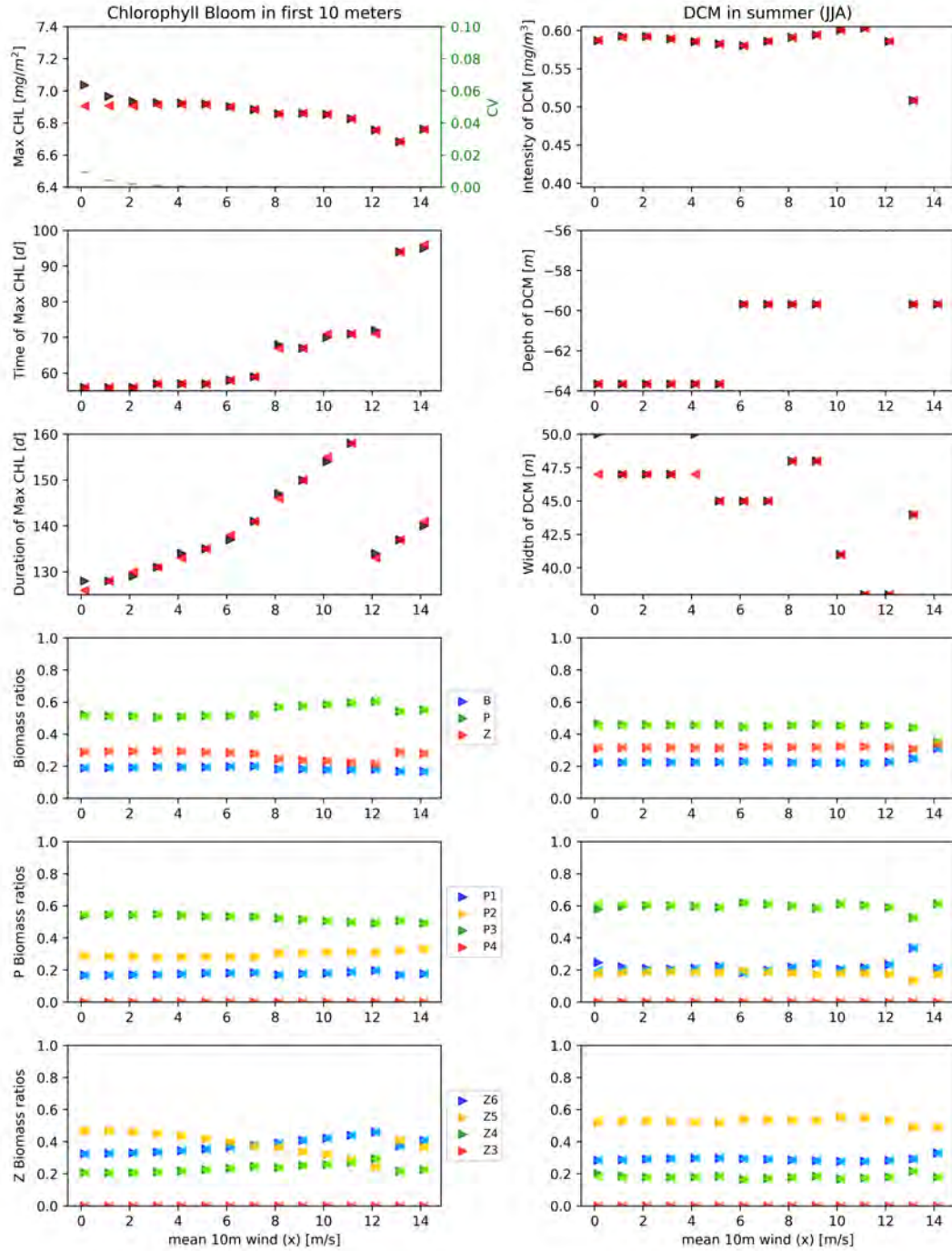
Fig. S1. Bifurcation diagrams for the dynamic regimes associated to Chlorophyll bloom (left panels) and DCM (right panels) under the variation of the wind forcing in the EXP-SEQ experimental setup. For each column, in the first three panels from the top the black triangles stand for the simulations which follow the x-axis values with time (forward, from original to extreme environmental condition), the red triangle the simulations which go backwards (from extreme to original environmental conditions). For each column, in the first three panels from the bottom the darker coloured triangles stand for the simulations which follow the x-axis values with time, the lighted coloured triangles the simulations which go backwards, e.g. blue goes forward and light blue goes backward. The reversibility has been quantified with CV < 0.1 , shown in green.
