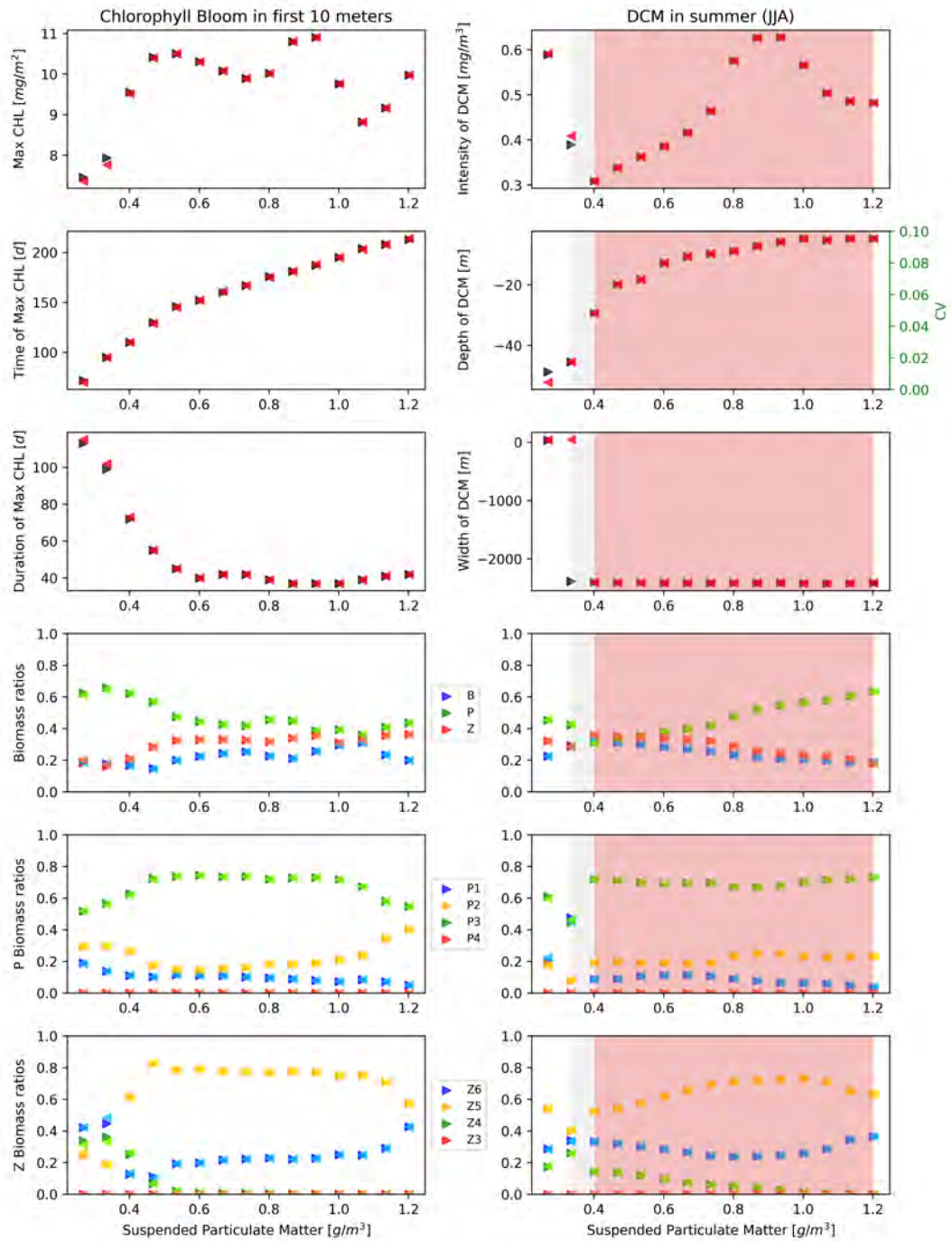
Fig. S7. Bifurcation diagrams for the dynamic regimes associated to Chlorophyll bloom (left panels) and DCM (right panels) under the variation of the suspended particulate matter (SPM) forcing in the EXP-SEQ experimental setup. For each column, in the first three panels from the top the black triangles stand for the simulations which follow the x-axis values with time (forward, from original to extreme environmental condition), the red triangle the simulations which go backwards (from extreme to original environmental conditions). For each column, in the first three panels from the bottom the darker coloured triangles stand for the simulations which follow the x-axis values with time, the lighted coloured triangles the simulations which go backwards, e.g. blue goes forward and light blue goes backward. In the right panels the shaded region corresponds to the values of the 'Width of DCM' which identifies when the DCM does not exist anymore, i.e. DCM loses its structure and the chlorophyll is spread along the water column. A grey shade and a red shade are superimposed highlighting the absence of the DCM in both the forward and backward simulations. The reversibility has been quantified with CV < 0.1 , shown in green.
