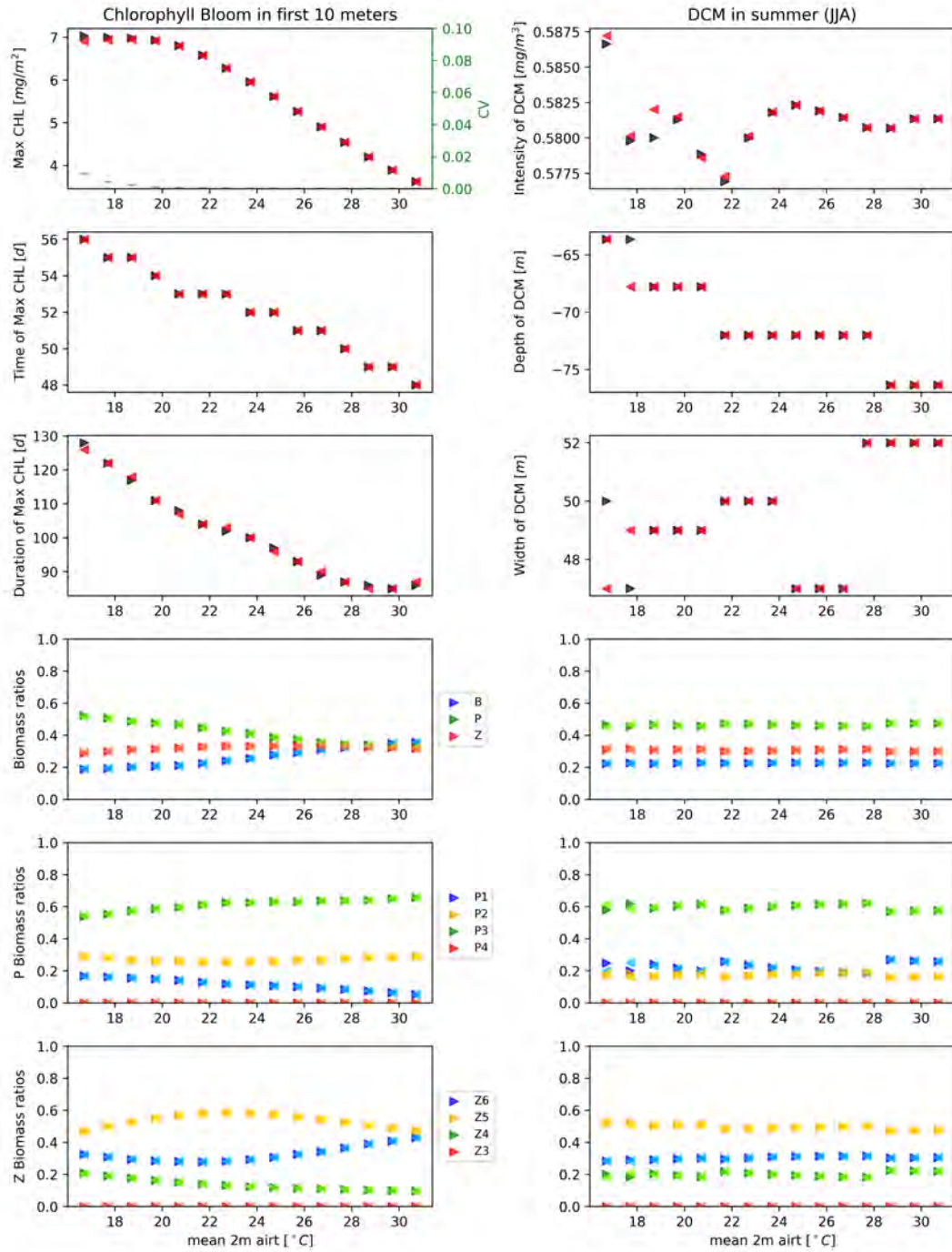
Fig. S3. Bifurcation diagrams for the dynamic regimes associated to Chlorophyll bloom (left panels) and DCM (right panels) under the variation of the air temperature forcing in the EXP-SEQ experimental setup. For each column, in the first three panels from the top the black triangles stand for the simulations which follow the x-axis values with time (forward, from original to extreme environmental condition), the red triangle the simulations which go backwards (from extreme to original environmental conditions). For each column, in the first three panels from the bottom the darker coloured triangles stand for the simulations which follow the x-axis values with time, the lighted coloured triangles the simulations which go backwards, e.g. blue goes forward and light blue goes backward. The reversibility has been quantified with CV < 0.1 , shown in green.
