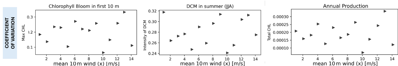
Figure 8. Bifurcation diagrams showing the response of the model's dynamic regimes to the perturbation of the model parameters under the increase in wind forcing (EXP-BGC, presented in Sect. 2.4.4). The y axis shows the coefficient of variation (CV) of the dynamic regimes over the ensemble of simulations with different parameters. The CV of the annual production dynamics regimes (rightmost panel) is 3 orders of magnitude lower than that of the seasonal dynamic regimes (first two panels).
