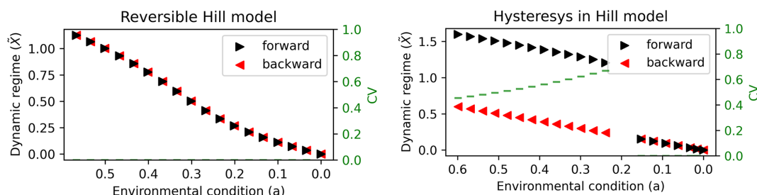
Figure 2. Bifurcation diagrams showing the response of the Hill model's dynamic regimes to the environmental condition a . The y axis value ( \bar{X} ) is the steady state solution of the Hill model (Eq. 1). The left panel shows a reversible response of the Hill model with parameters p = 2 and b = r = h = 1 , the forward path (black), from original to extreme environmental condition, and the backward path (red), from extreme to original environmental condition, follow the same trajectory satisfying CV < 0.1 . The right panel shows the hysteresis in the Hill model with parameters p = 18 (chosen to obtain a figure similar to the BFM outputs shown in the following) and b = r = h = 1 , the forward path (black), from original to extreme environmental condition, and the backward path (red), from extreme to original environmental condition, follow different trajectories satisfying CV > 0.1 .
