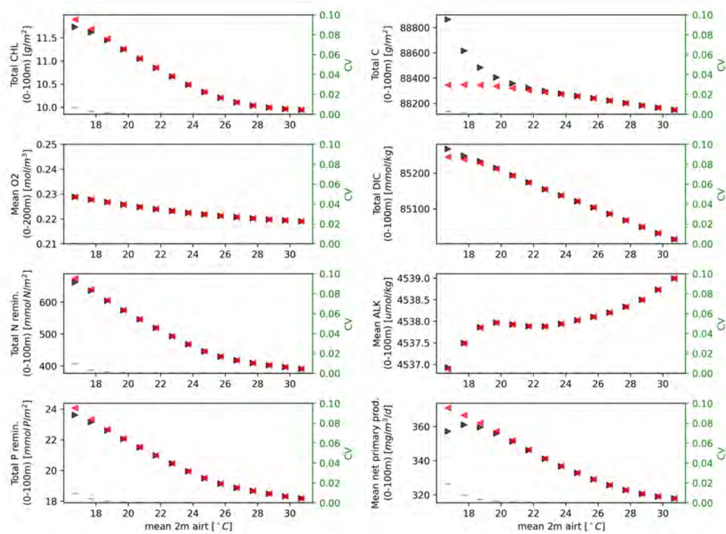
Fig. S4. Bifurcation diagrams under the variation of air temperature forcing in the EXP-SEQ experimental setup for the dynamic regimes associate with annual production and recycling. The black triangles stand for the simulations which follow the x-axis values with time (forward, from original to extreme environmental condition), the red triangle the simulations which go backwards (from extreme to original environmental conditions). The reversibility has been quantified with CV < 0.1 , shown in green.
