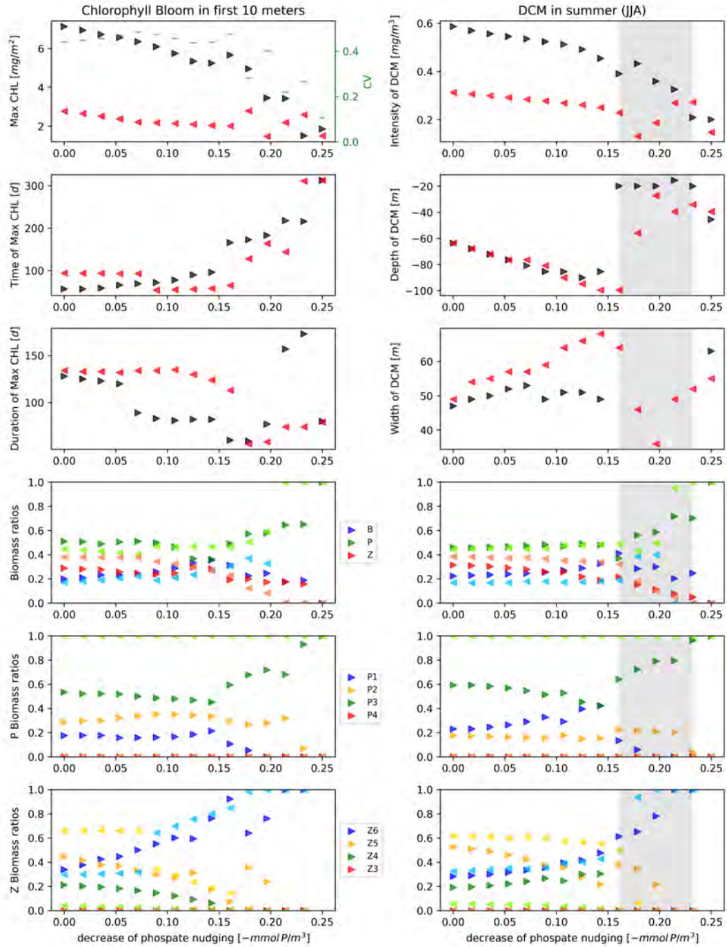
Fig. S5. Bifurcation diagrams for the dynamic regimes associated to Chlorophyll bloom (left panels) and DCM (right panels) under the variation of the phosphate nudging forcing in the EXP-SEQ experimental setup. For each column, in the first three panels from the top the black triangles stand for the simulations which follow the x-axis values with time (forward, from original to extreme environmental condition), the red triangle the simulations which go backwards (from extreme to original environmental conditions). For each column, in the first three panels from the bottom the darker coloured triangles stand for the simulations which follow the x-axis values with time, the lighted coloured triangles the simulations which go backwards, e.g. blue goes forward and light blue goes backward. In the right panels the shaded region corresponds to the values of the 'Width of DCM' which identifies when the DCM does not exist anymore, i.e. DCM loses its structure and the chlorophyll is spread along the water column. The grey shade highlight the absence of the DCM only in the forward simulations. The hysteresis has been quantified with CV > 0.1 , shown in green.
