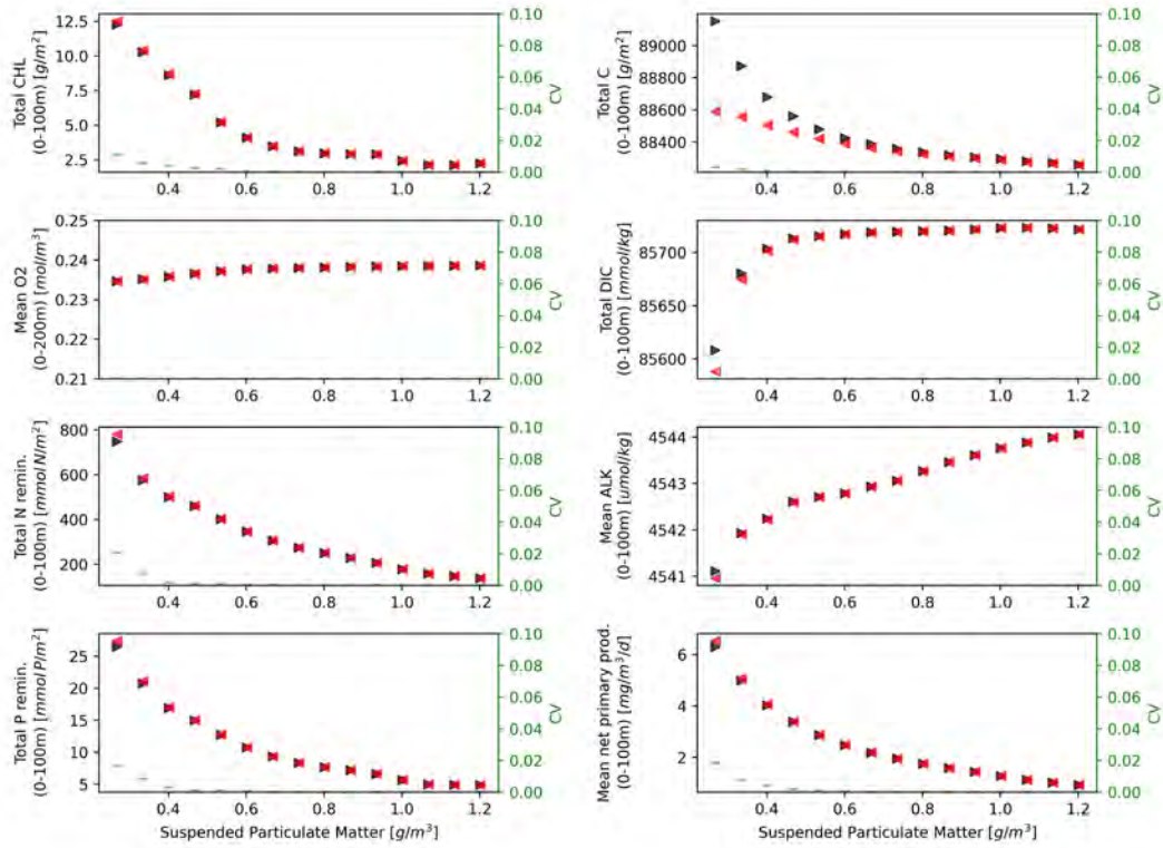
Fig. S8. Bifurcation diagrams under the variation of suspended particulate matter (SPM) forcing in the EXP-SEQ experimental setup for the dynamic regimes associate with annual production and recycling. The black triangles stand for the simulations which follow the x-axis values with time (forward, from original to extreme environmental condition), the red triangle the simulations which go backwards (from extreme to original environmental conditions). The reversibility has been quantified with CV < 0.1 , shown in green.
