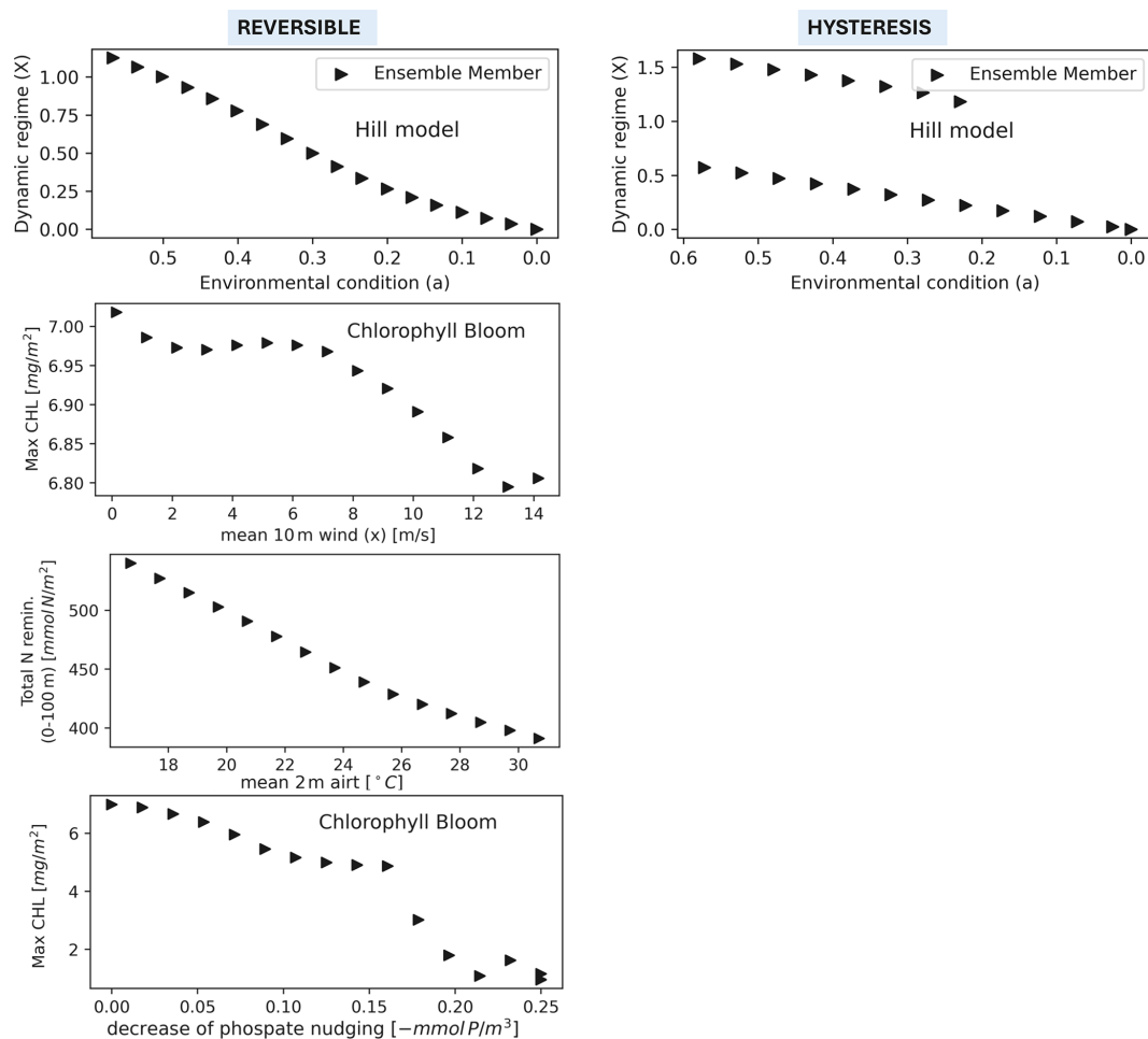
Figure 6. EXP-INI setup: Bifurcation diagrams showing the response of the model's dynamic regimes to environmental forcings. The mean magnitude of the environmental forcings ( x axis) goes from its original value (left) to extreme values (right). The left panels show a reversible response: for each value of the environmental forcings all the ensemble members with different initial conditions visit the same dynamic regime (only one triangle). The right panels show the hysteresis, for some values of the environmental forcings different ensemble members visit different dynamic regimes (two triangles in column). The first row is a simplified representation of the response to environmental forcing using the Hill model (Scheffer et al., 2001), where a is a parameter of the model. The methodology is presented in Sect. 2.4.2. The other rows show the response of the dynamic regimes to the variation of 3 environmental forcings (wind, air temperature and phosphate nudging). Hysteresis never occurs for the studied forcings. CV is not shown because always smaller than 0.1.
