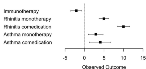
FIGURE 14 Regression coefficients.
