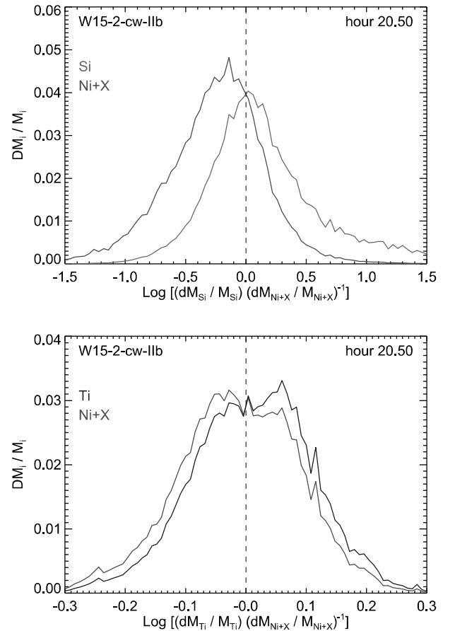
Fig. 2. Mass distribution of selected species versus the ratio R_{i,\text{Ni+X}} = \log[(dM_i/M_i)(dM_{\text{Ni+X}}/M_{\text{Ni+X}})^{-1}] (where i stands for Si or Ti) at t \approx 20.5\text{ h} after core bounce for model W15-2-cw-IIb (Wongwathanarat et al. 2017). The quantity [Ni + X] denotes ( ^{56}\text{Ni} + 0.5\text{ }^{56}\text{X} ).
