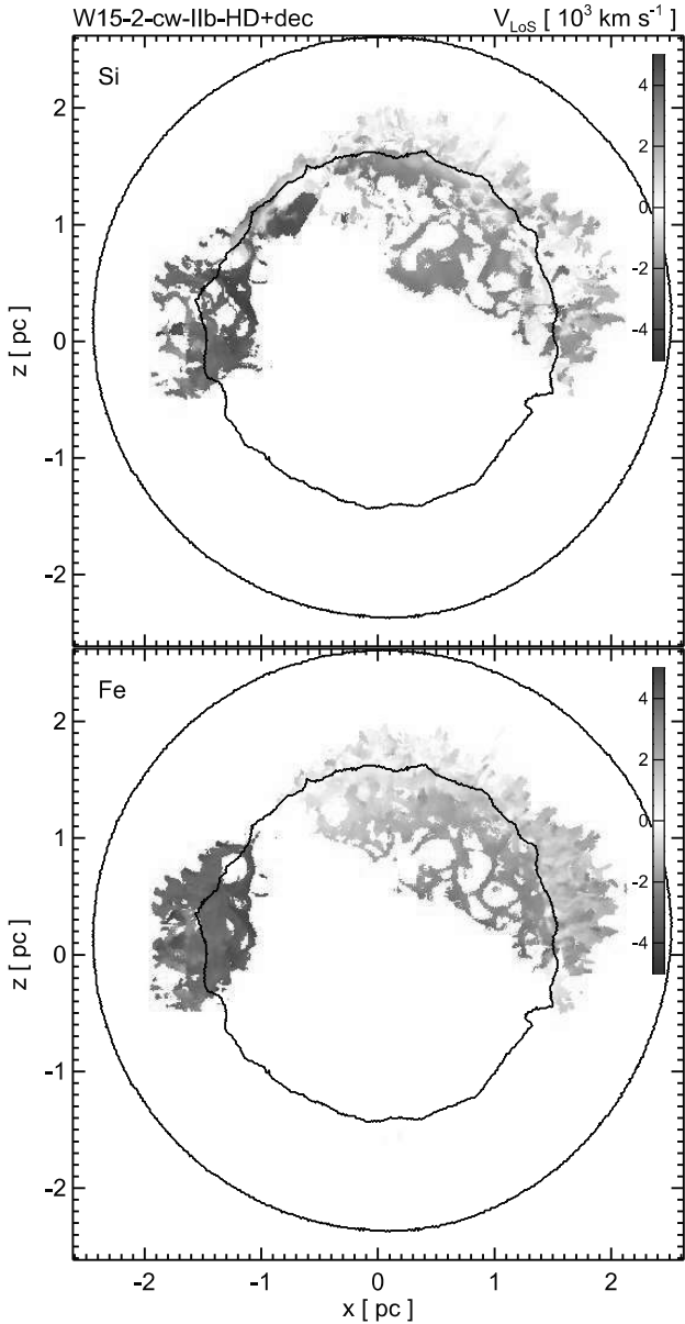
Fig. 19. Maps of average EM-weighted velocity along the LoS for shocked Si ( upper panel ) and Fe ( lower panel ) at the age of Cas A for model W15-2-cw-11b-HD+dec. The approximate velocity range is \pm 5000 \text{ km s}^{-1} (see color bar on the right in units of 1000 \text{ km s}^{-1} ). The solid contours mark the cuts of the forward and reverse shocks in the plane of the sky passing through the center of the explosion. These images correspond to the effective Doppler maps derived from observations.
