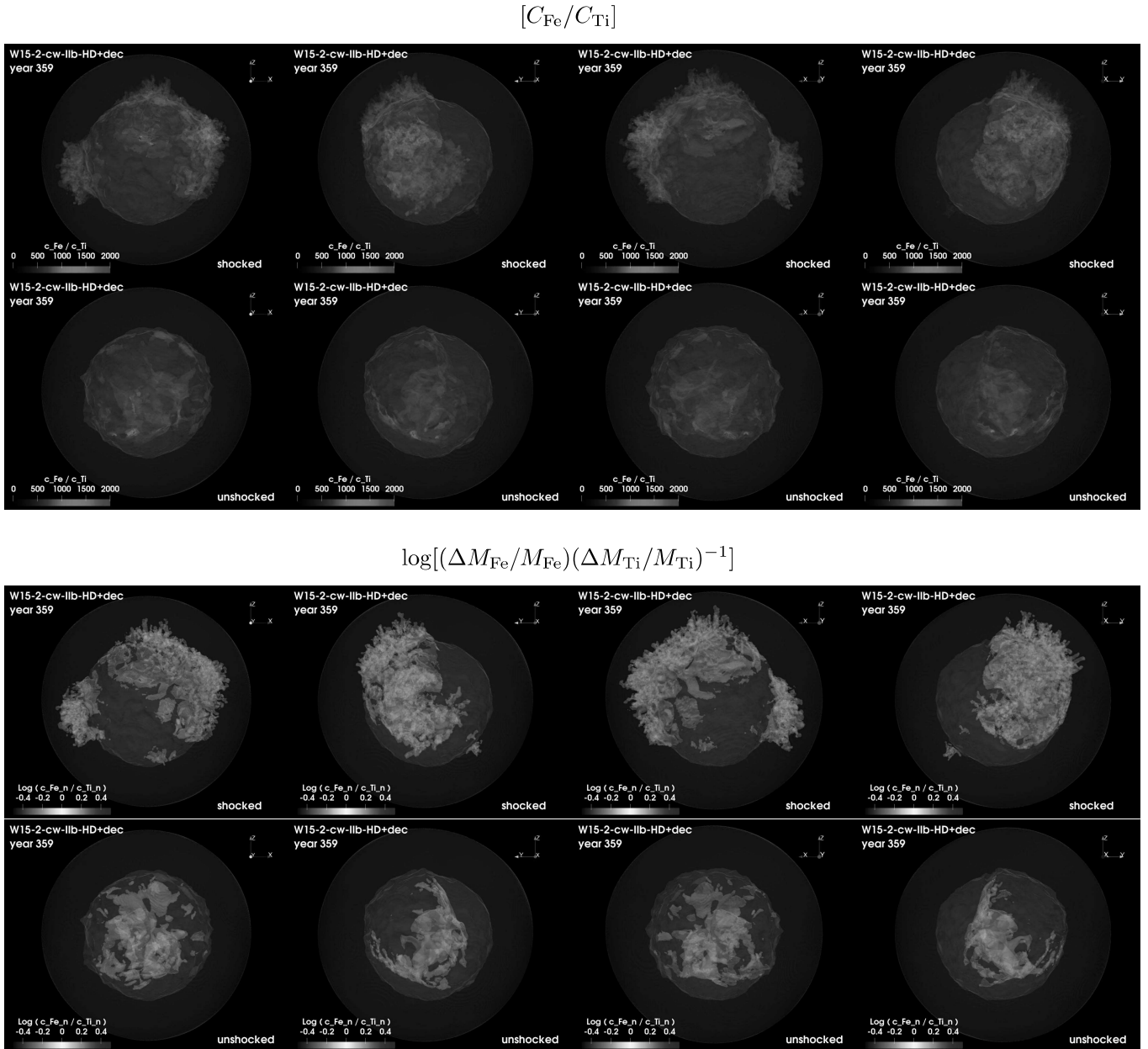
Fig. 15. 3D distributions of mass fraction ratio [C_{\text{Fe}}/C_{\text{Ti}}] (upper 2 rows) and log of abundance ratio, \log[(\Delta M_{\text{Fe}}/M_{\text{Fe}}) \times (\Delta M_{\text{Ti}}/M_{\text{Ti}})^{-1}] (lower 2 rows), for different viewing angles (from left to right) for model W15-2-cw-IIb-HD+dec at the age of Cas A. The results for both shocked and unshocked ejecta are shown. The two semi-transparent quasi-spherical gray isosurfaces indicate the forward (outermost surface) and reverse (inner surface) shocks. The ratios are calculated in cells with density of Fe and Ti greater than 5% of the maximum density of the respective species. See online Movie 4 for an animation of these data; a navigable 3D graphic of the abundance ratio, \log[(\Delta M_{\text{Fe}}/M_{\text{Fe}}) \times (\Delta M_{\text{Ti}}/M_{\text{Ti}})^{-1}] , in log scale, at the age of Cas A is available at https://skfb.ly/6XnFJ .
