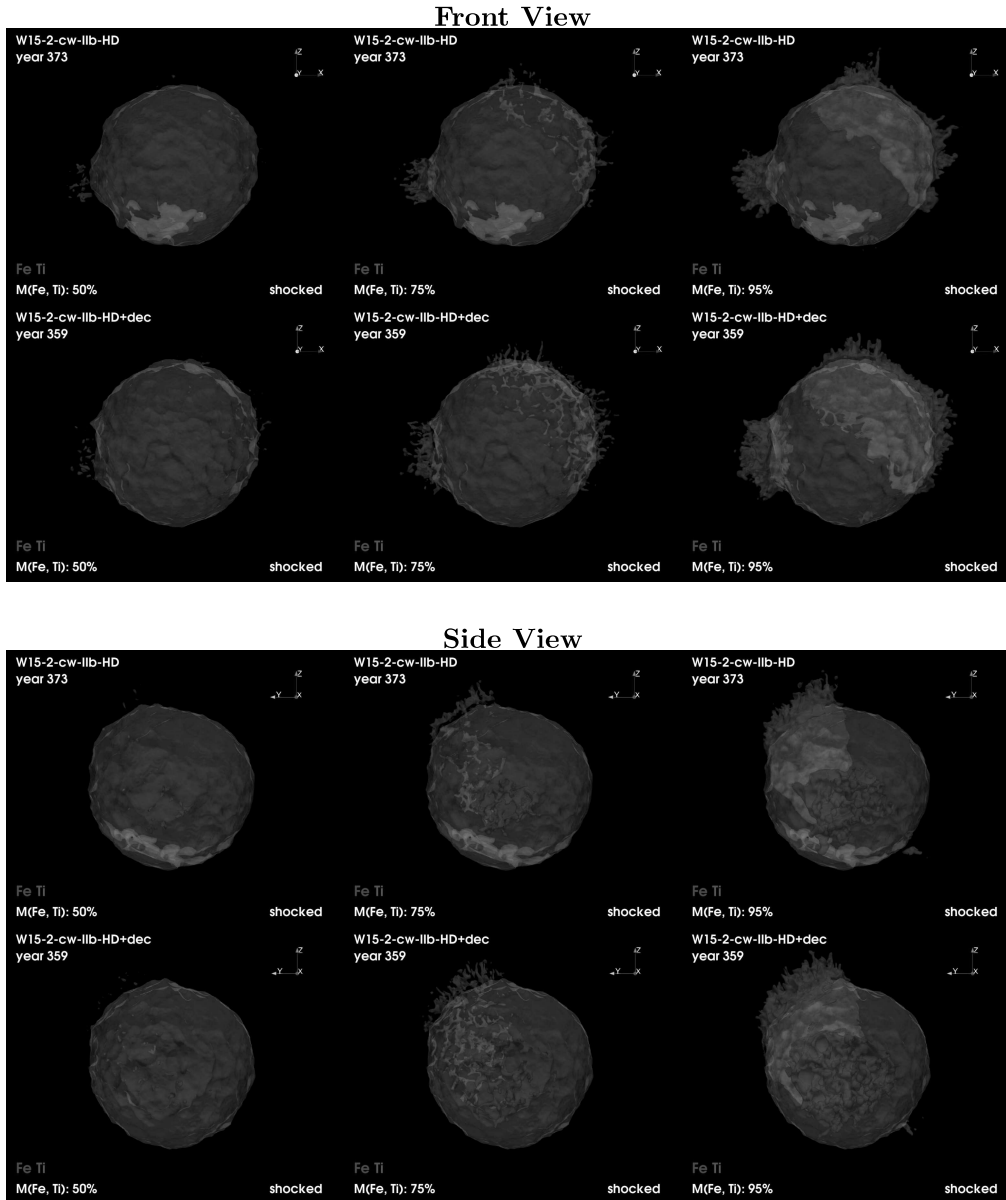
Fig. 14. Same as in Fig. 12, but for the distributions of shocked Fe (red) and Ti (blue). The values of the mass fractions are selected so that the corresponding isosurfaces enclose, from left to right , 50, 75, and 95% of the total mass of the respective shocked species. The red isosurfaces correspond to a value of Fe density in model W15-2-cw-IIb-HD (W15-2-cw-IIb-HD+dec) which is, in units of 10^{-25} \text{ g cm}^{-3} , 72 (50), 35 (26), 7.5 (7.9), respectively; the blue isosurfaces correspond to a value of Ti density in model W15-2-cw-IIb-HD (W15-2-cw-IIb-HD+dec) which is, in units of 10^{-26} \text{ g cm}^{-3} (considering the tracer-particle-based post-processing with a large nuclear network, Wongwathanarat et al. 2017, but not considering its decay in ^{44}\text{Ca} ), 21 (15), 10 (7.9), 2.8 (2.5), respectively (considering the decay of ^{44}\text{Ti} in ^{44}\text{Ca} , these values are scaled by a factor of 0.027, for an e-folding time of 90 yr). A navigable 3D graphic of these distributions is available at https://skfb.ly/6UMxI .
