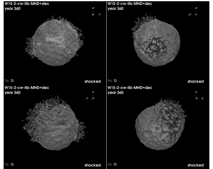
Fig. B.3. Same as in Fig. 8, but for model W15-2-cw-IIb-MHD+dec.
