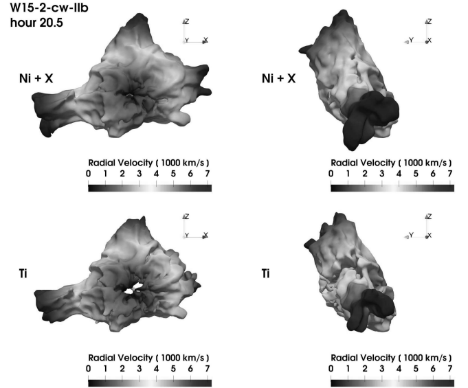
Fig. 1. Isosurfaces of mass fractions of ( ^{56}\text{Ni} + 0.5\text{ }^{56}\text{X} ) (upper panels) and ^{44}\text{Ti} (lower panels) from different viewing angles for model W15-2-cw-IIb at t = 20.5\text{ h} after core bounce (from Wongwathanarat et al. 2017). The isosurfaces correspond to a value of mass fraction which is at 30% of the peak mass fraction of each species. The colors give the radial velocity in units of 1000\text{ km s}^{-1} on the isosurface; the color coding is defined at the bottom of each panel.
