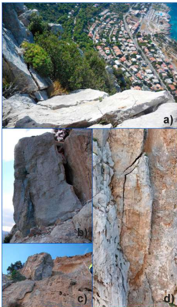
Figure 5. Unstable blocks as a. slabs, b.,c.boulders and d. pinnacles which could involve in kinematics of toppling.
