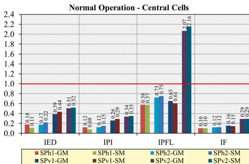
Fig. 24. RCC-MRx criteria evaluation within global model and CC sub-model in NO scenario.
