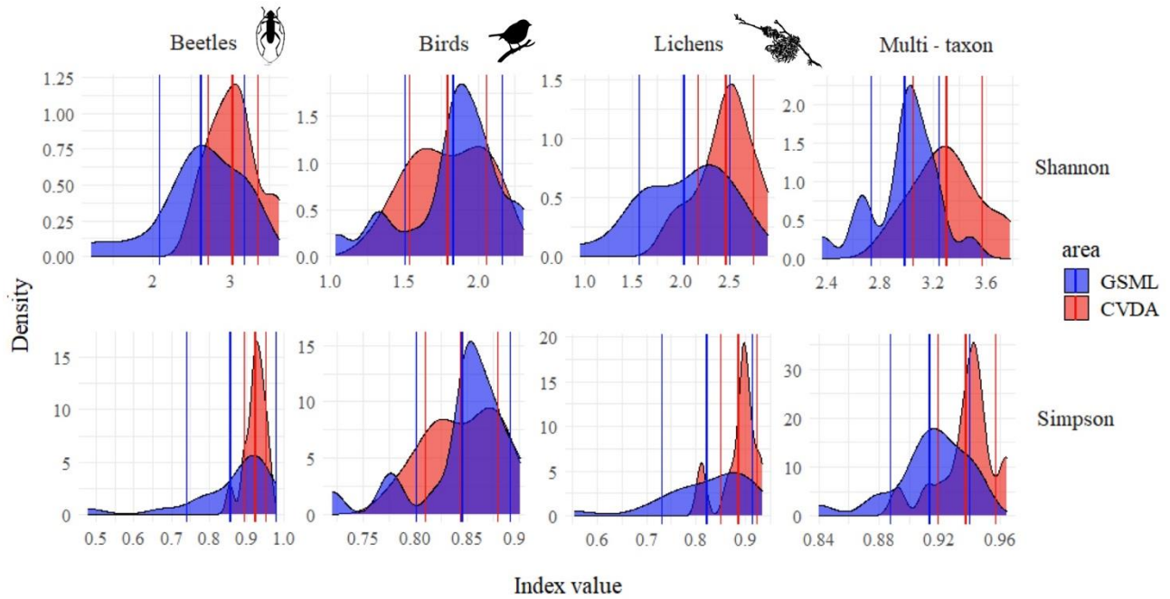
Supplementary Figure 1. Density plot of diversity indices for each study area for the whole communities and grouped by taxa. The thick vertical lines represent the mean and the thin ones the range of the standard deviation.
