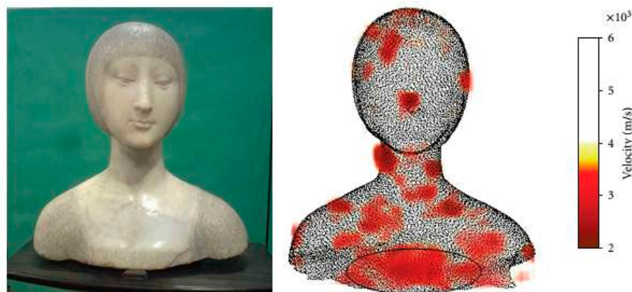
Figure 17. (Left) Bust of Eleonora d'Aragona (F. Laurana, 1468). (Right) Frontal 3D image with transparency of the investigated volume showing an area characterized by low P-wave velocity (or acoustic), corresponding to the support point of the bust [85].
