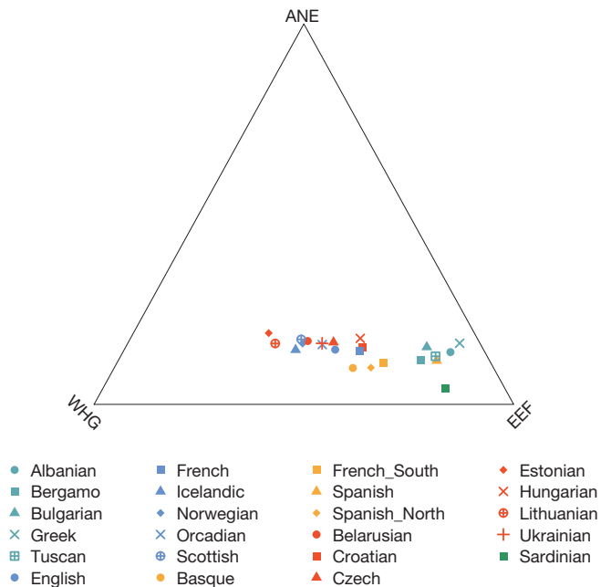
Figure 4 | Estimates of mixture proportions in present-day Europeans. Plot of the proportions of ancestry from each of three inferred ancestral populations (EEF, ANE and WHG).
