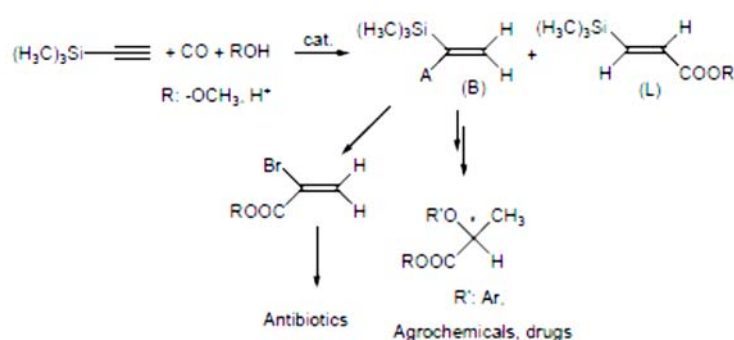
Scheme 1. Methoxy- and hydroxycarbonylation reaction of trimethylsilylacetylene.
