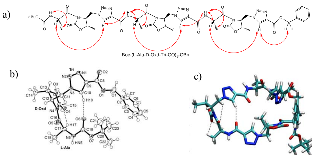
a) ROESY spectrum of Boc-(L-Ala-D-Oxd-Tri) 3 -OBn; b) Ortep-3 plot of Boc-L-Ala-D-Oxd-Tri-OBn; c) Most stable conformation of Boc-(L-Ala-D-Oxd-Tri) 3 -OBn by molecular dynamics.
