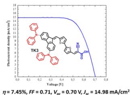
Fig. 1: TK3 structure and DSSC parameters .
