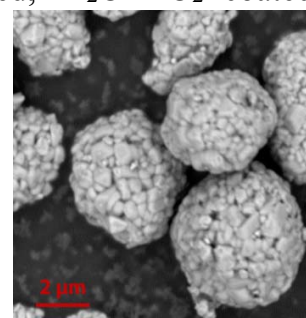
Fig.1 SEM image of coated NCA
