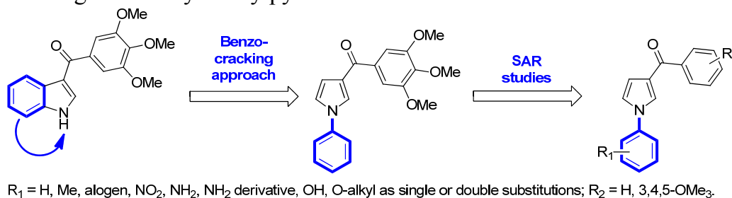
Chart 1. Design of 3-aroyle-1-arylpyrroles
