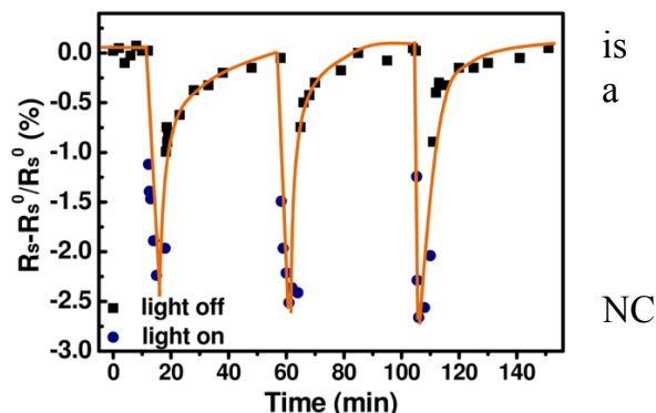
Figure. Monitoring of the change of the sheet resistance of graphene decorated with PBA-capped PbS NCs under three cycles of light irradiation with R_{s0} = 1000 \text{ Ohm}\times\text{sq}^{-1} the sheet resistance in the dark
