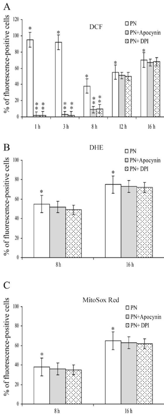
Figure 2. The effects of NOX inhibitors on DCF, DHE and MitoSox Red signals. Cells were treated for the indicated times with 25 \mu M parthenolide without or with 100 \mu M apocynin or 10 \mu M DPI, DCF, DHE and MitoSox Red signals were estimated as described in Materials and methods. The results are the mean \pm SE of three independent experiments. * P <0.01 vs. untreated control. ** P <0.01 vs. cells treated with only parthenolide. NOX, NADPH oxidase; DCF, dichlorofluorescein; DHE, dihydroethidium; DPI, diphenylpicrylhydrazolium.
