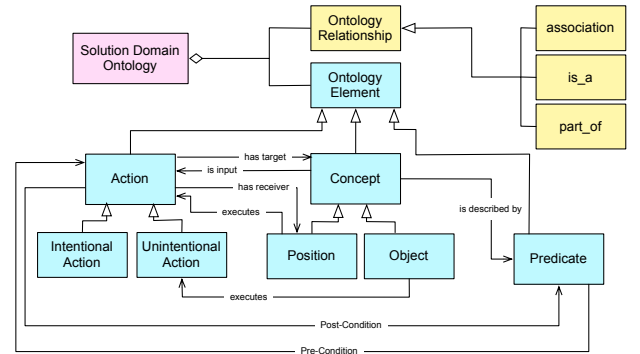
Fig. 2: The Problem Ontology Metamodel
