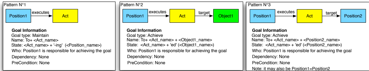
Fig. 4: Patterns Used for Identifying Goals
