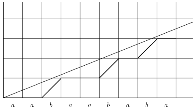
Fig. 1. The word s_{\alpha,0} .
