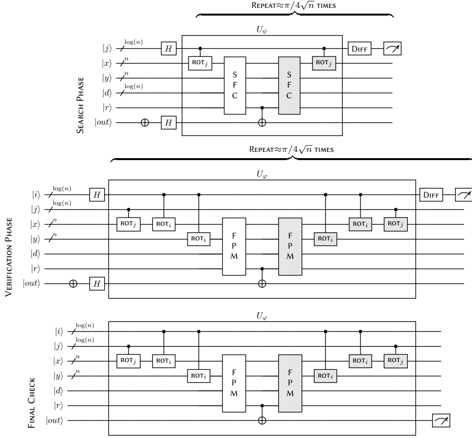
Figure 5: The quantum circuits implementing the three phases of the iterative test of the QUANTUM-LCS algorithm. For simplicity, the circuits do not contain all the ancillae qubits. The operators in gray color represent the inverse operators.
