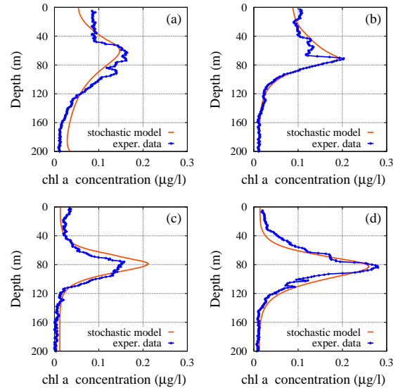
FIG. 1. Theoretical distributions (orange line) and experimental profiles (blue line) of the total chlorophyll a concentration. The numerical results, obtained by the stochastic model for \sigma_R = 0.0005 and \sigma_{b_i} = 0 , are compared with the experimental data collected in the sampling site ( 39^\circ 30'.00N , 13^\circ 30'.00E ), during the oceanographic surveys: VECTORM1, 24 November 2006 (panel a); VECTORM2, 3 February 2007 (panel b); VECTORM3, 22 April 2007 (panel c); VECTORM4, 9 June 2007 (panel d).
