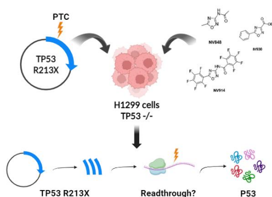
Figure 1: Experimental workflow for the study of the p53 rescue in H1299 p53 R213X cells by TRIDs molecule treatment
