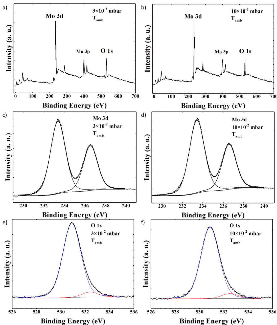
Figure 3. XPS spectra for \text{MoO}_x samples deposited at T_{\text{amb}} with \text{PO}_2 = 3 \times 10^{-2} mbar: (a) wide scan, (c) curve fitting of the Mo 3d spectrum, (e) curve fitting of the O 1s spectrum; and with \text{PO}_2 = 10 \times 10^{-2} mbar: (b) wide scan, (d) curve fitting of the Mo 3d spectrum, and (f) curve fitting of the O 1s spectrum.
