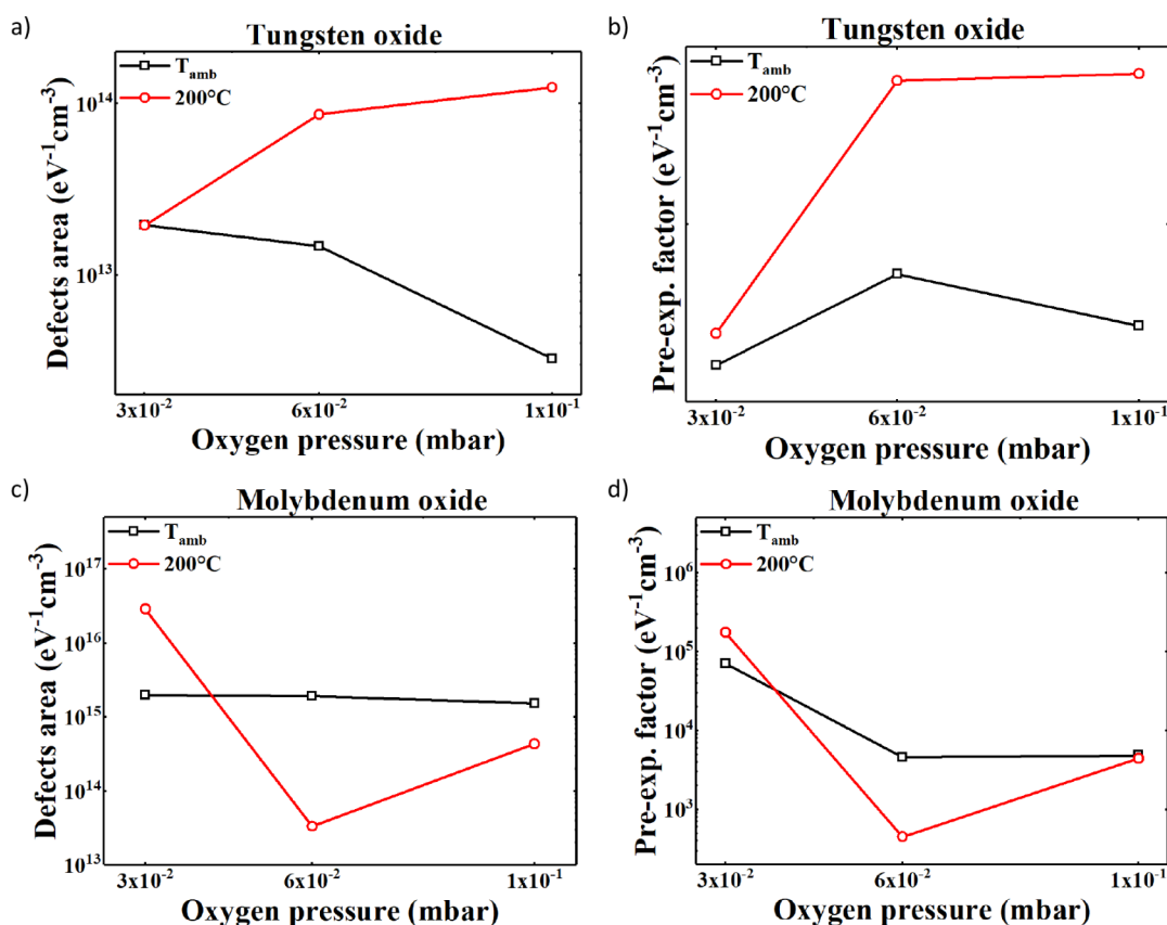
Figure 6. Resulting parameters for the samples under different deposition conditions: \text{WO}_x (a) A_D and (b) A_p ; \text{MoO}_x (c) A_D and (d) A_p .
