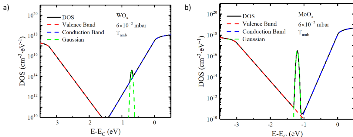
Figure 7. Resulting DOS (black line) with Gaussian defect distributions, the valence, conduction bands, and tails for the samples deposited at ambient temperature and 6 \times 10^{-2} mbar: (a) \text{WO}_x and (b) \text{MoO}_x .
