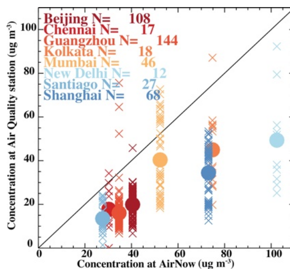
Figure 4. Comparison of \text{PM}_{2.5} observations from the US Embassy's AirNow network ( https://www.airnow.gov/international/us-embassies-and-consulates/ , last access: 10 June 2022) versus observations from the Chinese air quality network (downloaded from https://quotsoft.net/air/ , last access: 10 August 2022) (Beijing: 39.9^\circ\text{N} , 116.4^\circ\text{E} ; Guangzhou: 23^\circ\text{N} , 113^\circ\text{E} ; Shanghai: 31^\circ\text{N} , 121^\circ\text{E} ); from the Indian network ( https://app.cpcbcr.com/ccr/{#}/caaqm-dashboard-all/caaqm-landing/data , last access: 20 September 2022) (Chennai: 13^\circ\text{N} , 80^\circ\text{E} ; Kolkata: 23^\circ\text{N} , 88^\circ\text{E} ; New Delhi: 27^\circ\text{N} , 77^\circ\text{E} ); and from Santiago, Chile (Barraza et al., 2017) ( 23.7^\circ\text{S} , 70.4^\circ\text{W} ), from the Chilean air quality network ( https://sinca.mma.gob.cl/index.php/ , last access: 3 June 2022). The numbers after each city name are the number of stations found within 1^\circ distance from the AirNow (or Chile observation) station.
