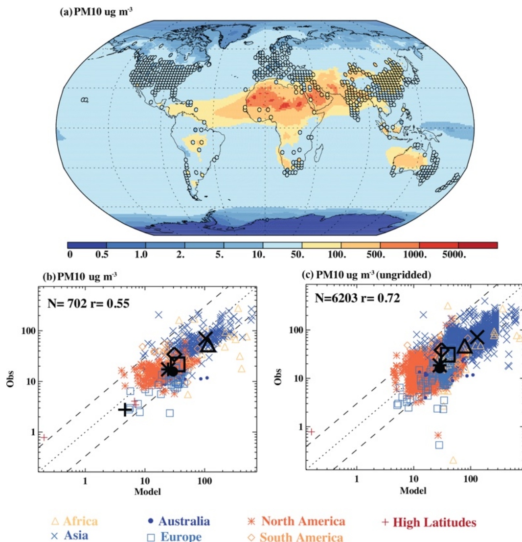
Figure 6. Model results and gridded observations for \text{PM}_{10} in \mu\text{g m}^{-3} , spatially mapped globally (a). A comparison of the model ( x axis) to the observations ( y axis) is shown for the gridded data (b) and including all stations (c). In the scatterplots, the colors and symbols indicate the regions, the bold black symbols are the average across each region (indicated by the symbol), the dotted line is the 1 : 1 line, and dashed lines are the factor-of-3 uncertainty estimates. More statistics are shown in Table S7, and maps focused on different regions are shown in Fig. S10.
