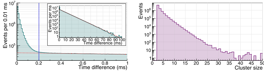
Fig. 10. (Left): Distribution of the time difference between electron events for measurement setting 1. Below 0.2 ms (shown by the solid blue line), there is a change in slope, indicating a contribution from correlated (i.e. clustered) events. The inset shows the time distribution for differences up to 100 ms. A fit to the distribution for 1\text{ms} < \Delta t < 100\text{ ms} is given by the red dashed line. (Right): Multiplicity distribution for the cluster events ( \Delta t < 0.2\text{ ms} ), excluding cluster sizes greater than 50. (For interpretation of the references to color in this figure legend, the reader is referred to the web version of this article.)
