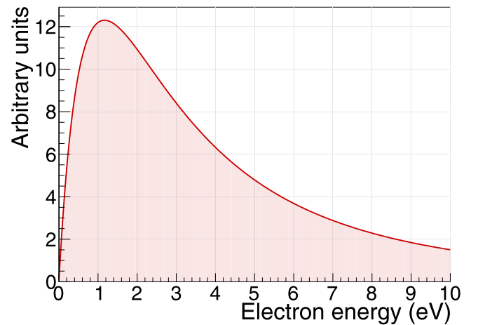
Fig. 6. Secondary-electron energy spectrum, calculated from Eq. (3) using a work function \Phi = 3.5 \text{ eV} .
