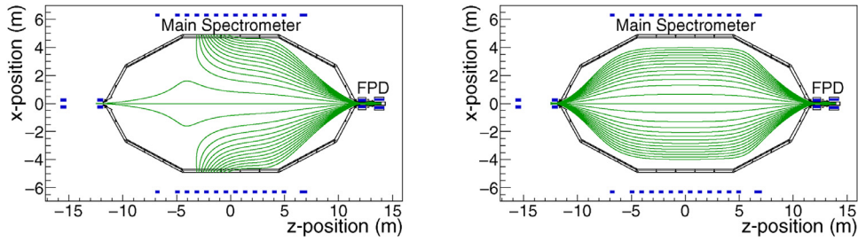
Fig. 4. (Left): Magnetic field lines used for setting 1 (“asymmetric” configuration). (Right): Magnetic field lines used for settings 2 and 3 (“symmetric” configuration). The displayed field lines intersect the FPD. Both configurations are rotationally symmetric about the spectrometer axis, but only the “symmetric” setting has reflection symmetry across the z = 0 plane. The blue rectangles indicate the positions of the air coils and the superconducting magnets at the MS entrance and exit. (For interpretation of the references to color in this figure legend, the reader is referred to the web version of this article.)
