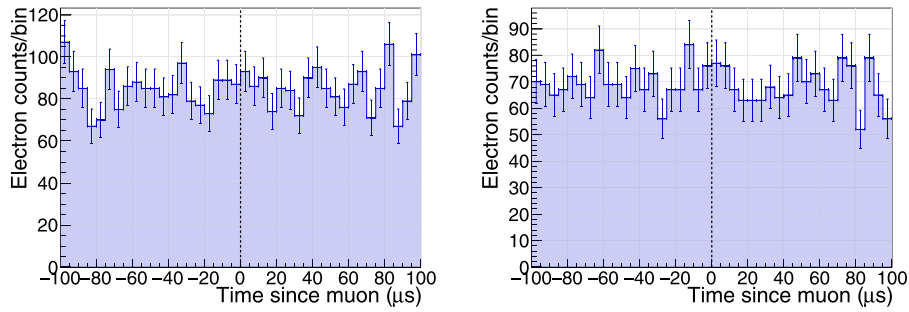
Fig. 7. The distribution of the time differences between electron and muon events. The black dashed line indicates t = 0 \mu\text{s} , the detection of a muon event. (Left): Field setting 2. (Right): Field setting 3.
