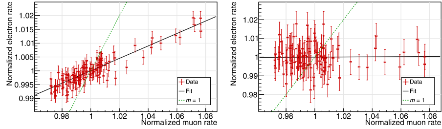
Fig. 11. (Left): Single electron rate ( M = 1 ) as a function of muon rate for setting 1. There is strong correlation ( r = 0.90 \pm 0.03 ), and the muon-induced fraction m is 0.225 \pm 0.010 . (Right): Cluster electron rate ( M \geq 3 ) as a function of muon rate for setting 1, showing no correlation ( r = 0.02 \pm 0.08 ). For both plots, the green dashed line represents the case of fully muon-induced background. (For interpretation of the references to color in this figure legend, the reader is referred to the web version of this article.)
