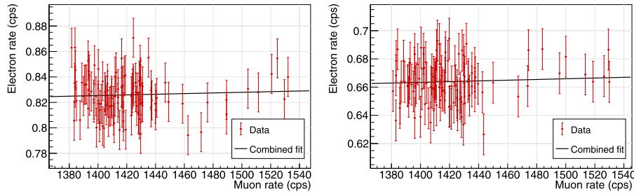
Fig. 12. Electron rate as a function of muon rate for setting 2 (left) and setting 3 (right). A simultaneous linear fit of both datasets (black line) finds a slope K = (2.5 \pm 3.2)10^{-5} , indicating m = 0.044 \pm 0.054 for setting 2 and m = 0.054 \pm 0.068 for setting 3.
