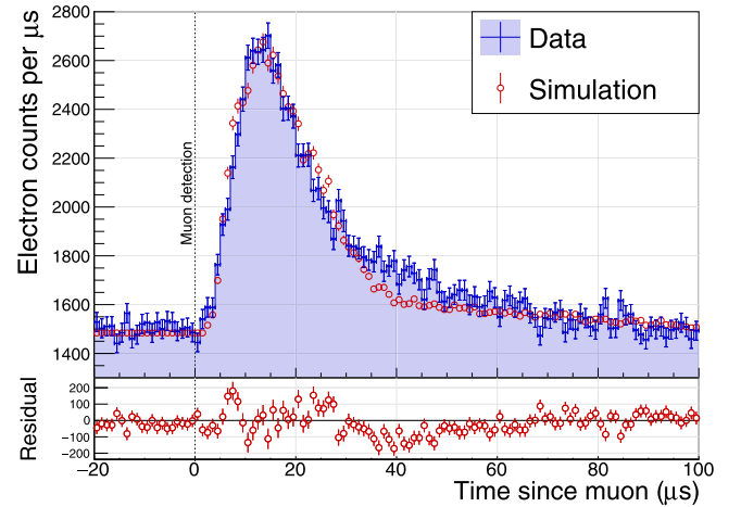
Fig. 5. The distribution of the time differences between electron and muon events collected with field setting 1 (blue points and fill). On the x-axis, t = 0 \mu\text{s} corresponds to the detection of a three-module muon event. Overlaid is the simulated time distribution (red markers) produced with KASSIOPEIA using the energy spectrum in Fig. 6 as input, with a maximum energy of 50 V \mu\text{eV} . The simulated distribution is scaled to minimize the \chi^2/\text{ndf} (248.0/99 for t > 0 \mu\text{s} ) with the offset from zero being fixed by the average electron counts prior to muon detection ( -100 \mu\text{s} < t < 0 \mu\text{s} ). The error bars are purely statistical. At the bottom of the figure, the residual (Simulation – Data) is displayed. (For interpretation of the references to color in this figure legend, the reader is referred to the web version of this article.)
