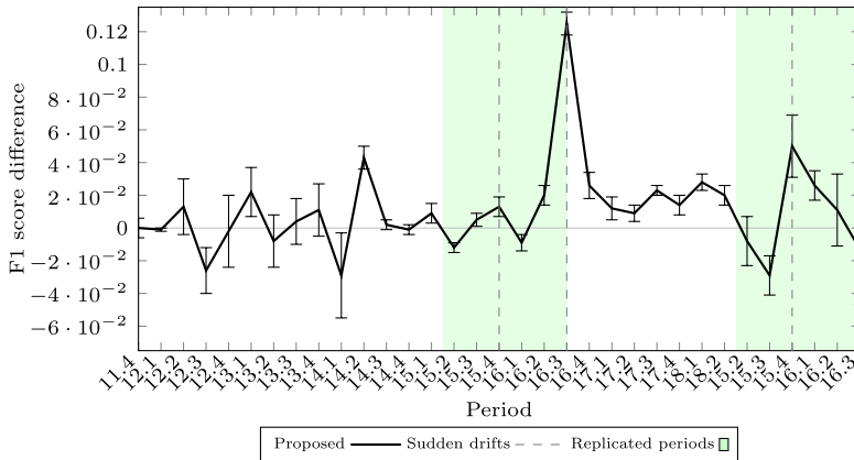
Fig. 10 F1-score difference between the proposed system and the static classifier in the presence of additional artificial drifts. The self-evaluation agent, once trained, is able to recognize further drifts
