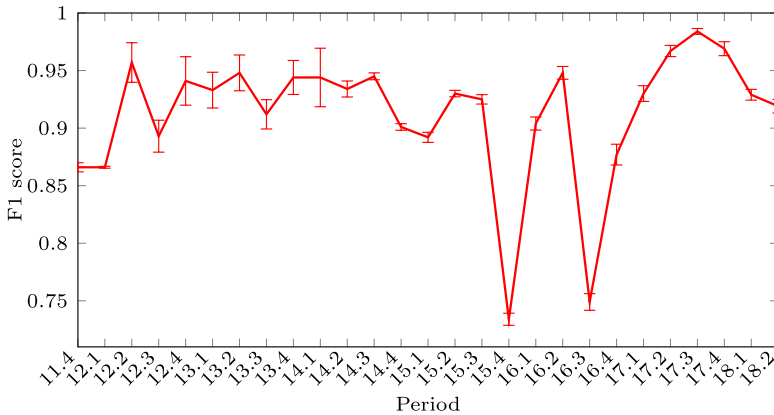
Fig. 9 Variance of the F1-score of the proposed system over the performed experiments
