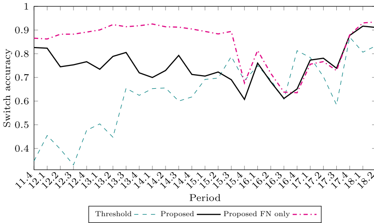
Fig. 12 Accuracy of the different techniques to detect local classifier's misclassifications and switch to the remote classifier. The self-evaluation agent effectively detects errors of the local classifier while the threshold approach is barely better than a random approach
