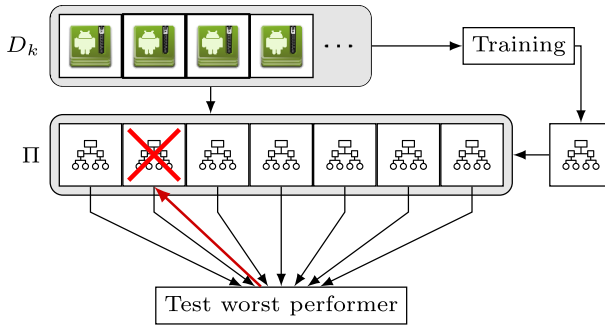
Fig. 4 Local classifier pool update mechanism: periodically, the worst classifier in the pool is removed. The removed classifier is replaced by a new classifier trained on the most recent data
