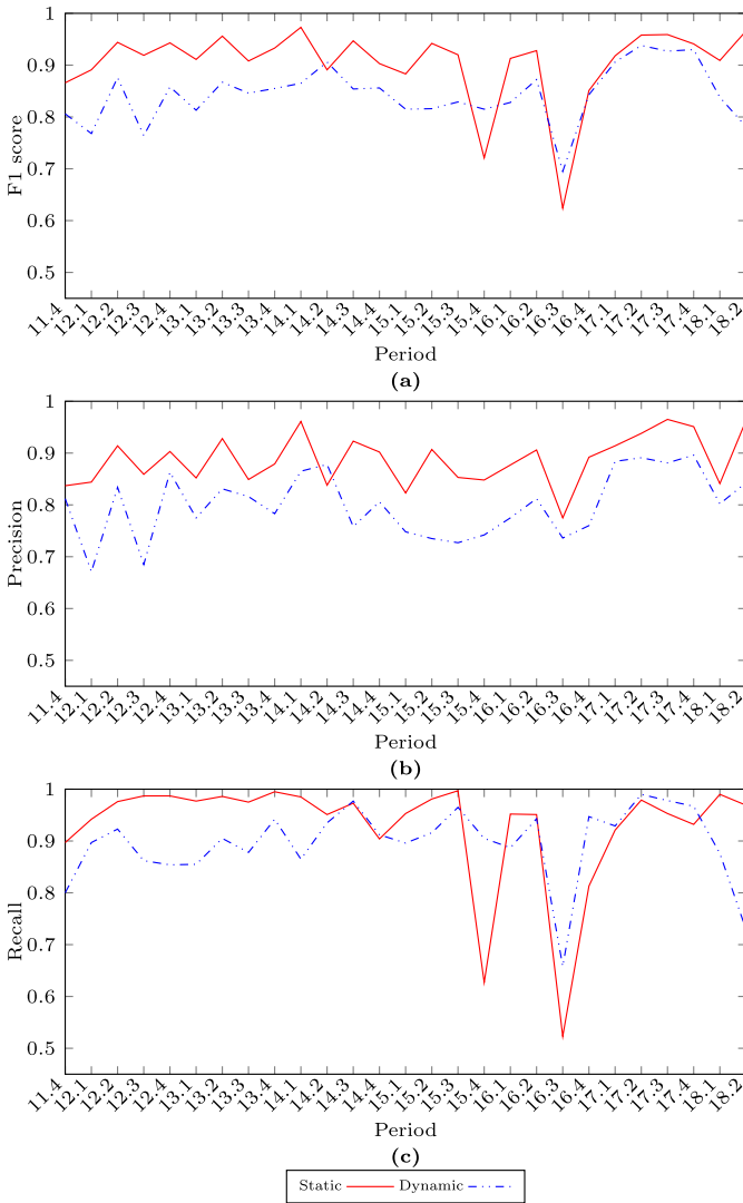
Fig. 6 Performance of the local and remote classifiers. When sudden drifts occur, the recall of the local classifier using static features is more heavily affected than the classifier using dynamic features
