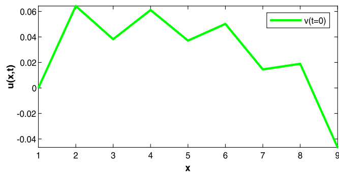
Fig. 5. Wave propagation of HSE for v(t=0) of case 1.
