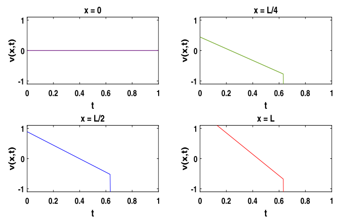
Fig. 6. Solution of HSE for different values of x for case 1.
