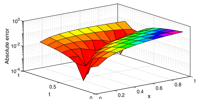
Fig. 10. Absolute errors of the HSE with \theta = 0.9 .
