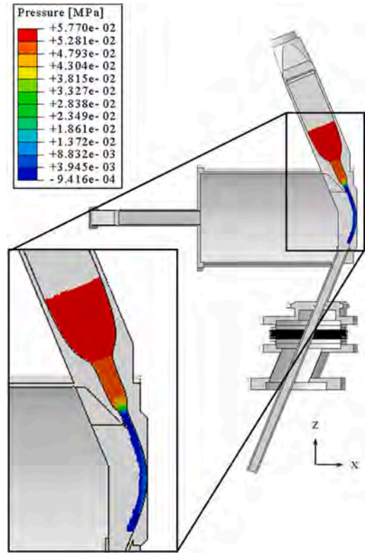
Fig. 7. Lithium static pressure spatial distribution.
