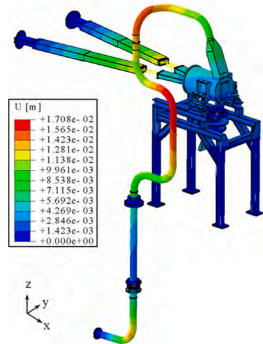
Fig. 11. Displacement field within TSY.
