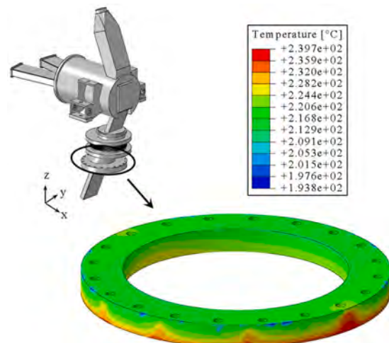
Fig. 4. Imposed temperature of the flange.
