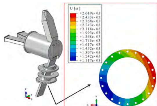
Fig. 8. Imposed total displacement field applied onto the QT flange.
