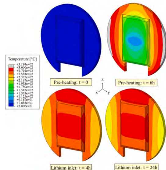
Fig. 14. Transient analysis: BPL thermal field - view1.
