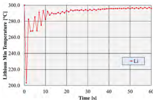
Fig. 16. Transient analysis: Minimum lithium temperature.
