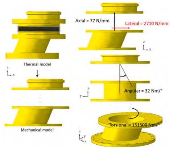
Fig. 10. ON bellows mechanical modelling.
