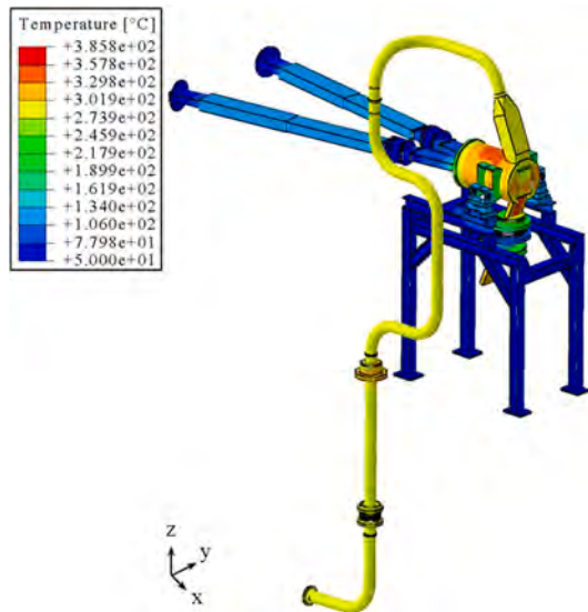
Fig. 5. Thermal field within TSY.
