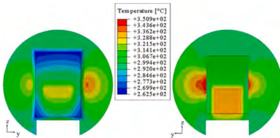
Fig. 6. Thermal field within the two sides of the BPL.
