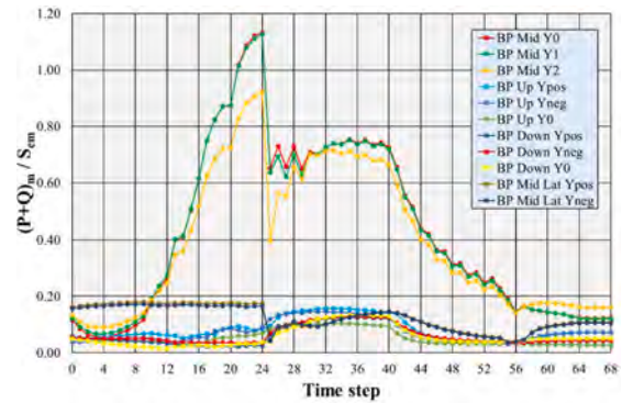
Fig. 22. Immediate plastic flow localization criterion results.
