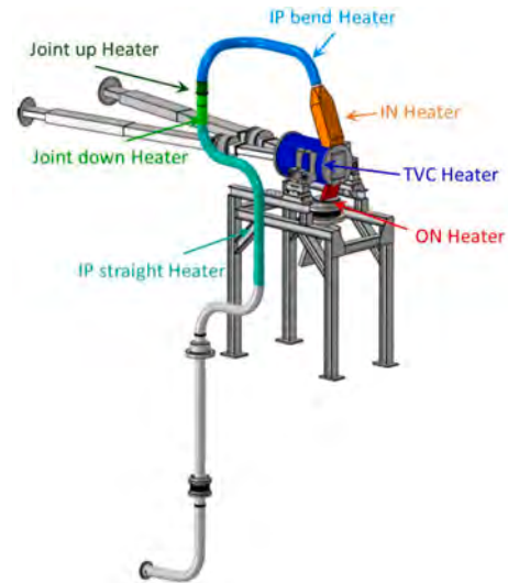
Fig. 13. Electric heaters surfaces and corresponding heat fluxes.
