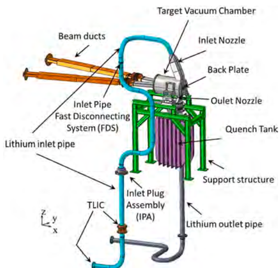
Fig. 1. The DONES Target System.
