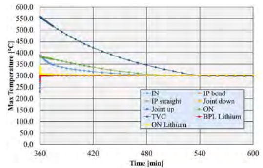
Fig. 18. Lithium inlet phase: Maximum temperature of the ON, BPL and heaters external surfaces.
