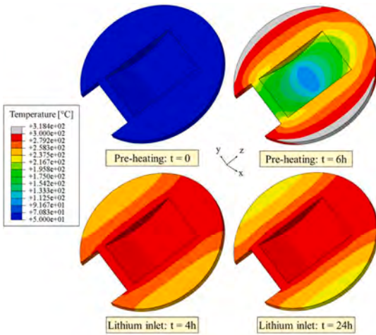
Fig. 15. Transient analysis: BPL thermal field - view2.
