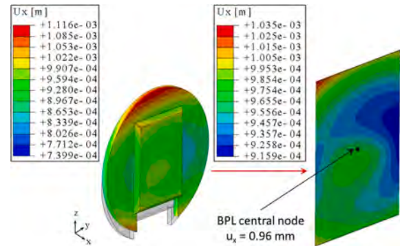
Fig. 12. BPL displacements along X direction and focus on the surface closest to the HFTM.
