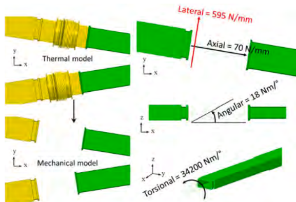
Fig. 9. BDs bellows mechanical modelling.
