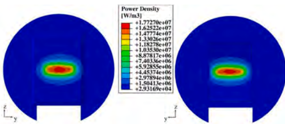
Fig. 3. Nuclear power density 3D field within the two sides of the BPL.
