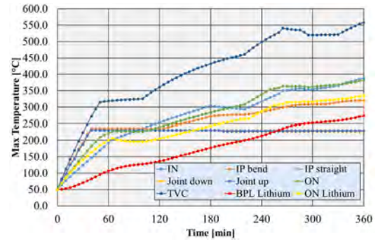
Fig. 17. Pre-heating phase: Maximum temperature of the ON, BPL and heaters external surfaces.
