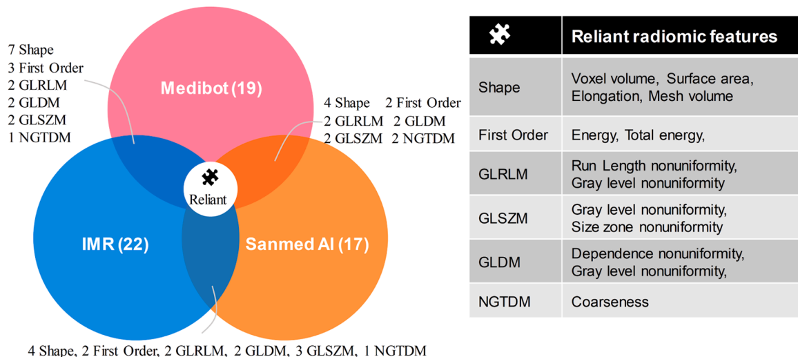
Fig. 7. Reliant radiomic features in survival status prediction.
