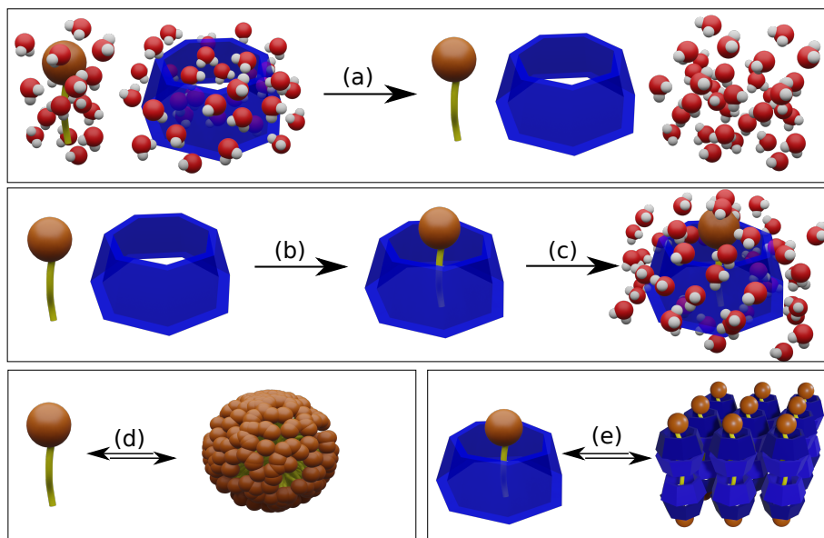
FIGURE 3.1: Schematic representation of the complex formation between surfactants and cyclodextrins in the steps it can be divided: (a) host and guest molecules are dehydrated; (b) the insertion of the surfactant molecule into the CD cavity takes place; (c) the CD/surfactant complex is, then, hydrated. In addition to these essential steps, the equilibrium (d) between the free surfactant and the ones in the micelles and (e) between the inclusion complexes and their assemblies has to be considered. Representation is out of scale. Reproduced from Ref. [9] with permission of Elsevier.
