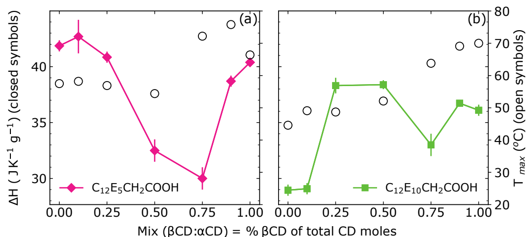
FIGURE 4.15: Enthalpy \Delta H (J K -1 g -1 surf ) and temperature transitions extracted from thermograms of the C_{12}E_5CH_2COOH and C_{12}E_{10}CH_2COOH with \alpha -cyclodextrin and \beta -cyclodextrin and their mixtures. Unpublished data.
