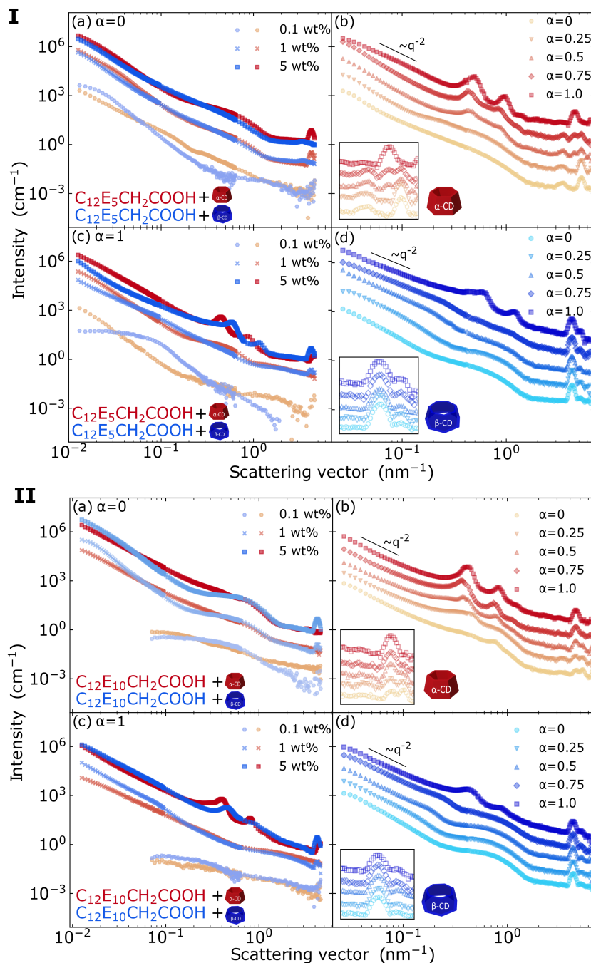
FIGURE 4.8: SANS curves profiles of C_{12}E_5CH_2COOH (I) and C_{12}E_{10}CH_2COOH (5 %wt surfactant) (II) with \alpha CD and \beta CD. SANS intensity is expressed as a function of the scattering vector ( q ). The measurements at (a) \alpha = 0 and (c) \alpha = 1 and the different degrees of ionization for (b) \alpha CD and (d) \beta CD. Curves are scaled by successive factors of 10 to improve readability. The insets represent an enlargement of the high q region. Data were acquired at D11@ILL and the degree of ionization, at the D22@ILL.
