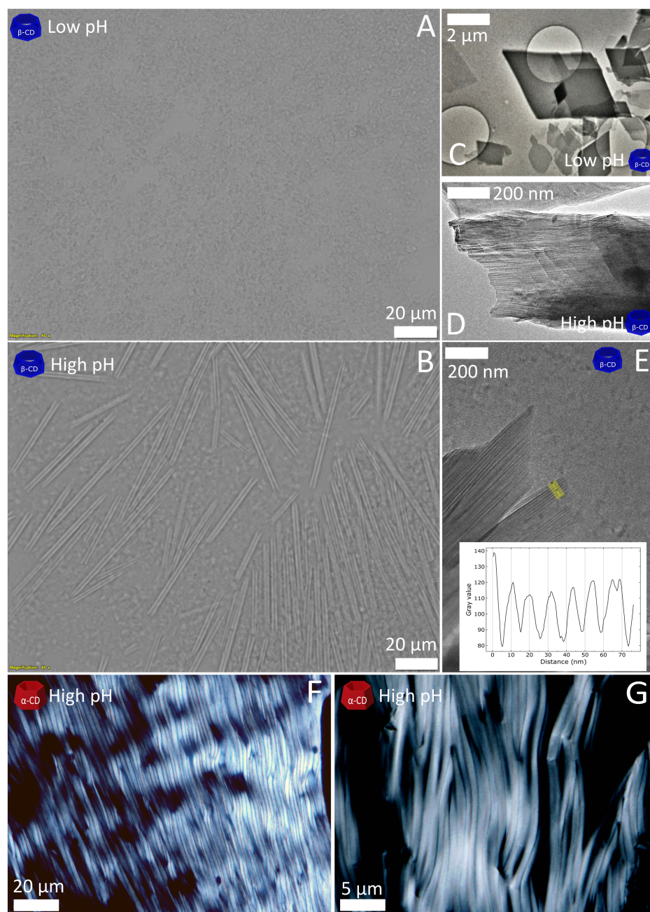
FIGURE 4.10: Morphology of the inclusion complexes aggregates observed by microscopy. Aggregates verified for \text{C}_{12}\text{E}_5\text{CH}_2\text{COOH} - 2\beta\text{CD} inclusion complexes. Optical microscopy overview of the assemblies obtained at (a) \alpha = 0 and (b) \alpha = 1 (scale bar: 20 \mu\text{m} ). (c) TEM image of the rhombic structures from the assembly with the nonionic surfactant (scale bar: 2 \mu\text{m} ). (d) Cryo-TEM pictures of the tubular structure edge obtained from \alpha = 1 (scale bar: 200 nm) and (e) Cryo-EM picture zoom-in of the multi-layered tube wall (scale bar: 200 nm). Polarized optical microscopy images of \alpha\text{CD} systems: (f) Ionized \text{C}_{12}\text{E}_5\text{CH}_2\text{COOH} - \alpha\text{CD} (scale bar: 20 \mu\text{m} ) and (g) Ionized \text{C}_{12}\text{E}_{10}\text{CH}_2\text{COOH} - \alpha\text{CD} (scale bar: 5 \mu\text{m} ). Reproduced from Ref. [84] with permission of the Royal Society of Chemistry.
