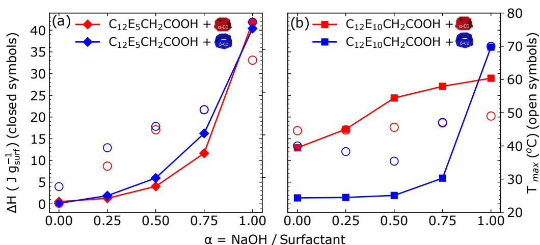
FIGURE 4.13: The enthalpic changes \Delta H ( \text{J g}^{-1}_{\text{surf}} ) as a function of the surfactant's degree of ionization for (a) \text{C}_{12}\text{E}_5\text{CH}_2\text{COOH} ( \blacklozenge ) and (b) \text{C}_{12}\text{E}_{10}\text{CH}_2\text{COOH} ( \blacksquare ) systems and the temperature of the melting peak ( \circ ) corresponding to the assembled systems containing 5%wt surfactant with \alpha\text{CD} (red) and \beta\text{CD} (blue). Adapted from Ref. [120] with permission of the Royal Society of Chemistry.
