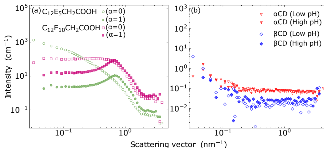
FIGURE 4.5: SANS curves of (a) C 12 E 5 CH 2 COOH and C 12 E 10 CH 2 COOH at 5%wt surfactant concentration and (b) α-cyclodextrin and β-cyclodextrin (saturated solutions) at α = 0 (open symbols) and α = 1 (closed symbols). Curves of the different surfactants are scaled by successive factors of 10 for readability. Data measured at ZOOM@ISIS.
