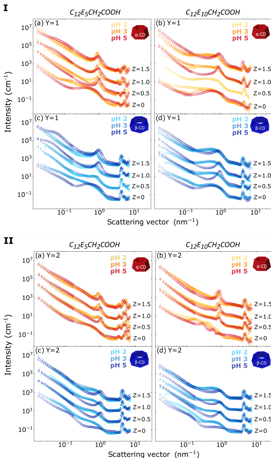
FIGURE 5.5: SANS patterns from chitosan-AEC-cyclodextrin complexes, recorded at pH 2, 3 and 5. At 2 %wt surfactant concentration, Z = 0, 0.5, 1.0 and 1.5 at (I) CD/surfactant ratio = 1 and (II) CD/surfactant ratio = 2. Chitosan systems with C_{12}E_5CH_2COOH with (a) \alpha CD and (c) \beta CD and C_{12}E_{10}CH_2COOH with (b) \alpha CD and (d) \beta CD. Successive curves are scaled by a factor of 15 for improved readability. Curves at pH 2 were recorded at D22 [119], and pH 3 and 5 were recorded at D11 (ILL, Grenoble). Curves which are not displayed were not measured due to precipitation.
