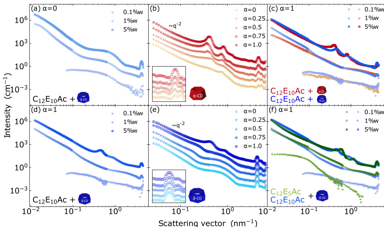
Fig. 5 At ratio CD/surfactant = 2, different concentrations of the \text{C}_{12}\text{E}_{10}\text{Ac} with \beta CD at (a) \alpha = 0 (nonionized), (d) \alpha = 1 (ionized). Different degree of ionization ( \alpha ) scattering profile curves of \text{C}_{12}\text{E}_{10}\text{Ac} with \alpha CD (b) and \beta CD (e). (c) Ionized surfactant with \alpha CD (red) and \beta CD (blue). (f) Comparison of \beta CD with ionized \text{C}_{12}\text{E}_5\text{Ac} (green) and \text{C}_{12}\text{E}_{10}\text{Ac} (blue) at different surfactant concentrations. Curves are scaled by successive factors of 7 for readability. Measurements of a, c, d and f were performed on D11 and b and e on D22 at ILL.
