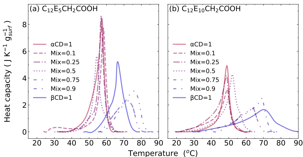
FIGURE 4.14: Thermograms of systems with a CD/Surfactant = 2, \Delta H ( \text{J K}^{-1} \text{g}_{\text{surf}}^{-1} ) corresponding to the inclusion complexes supramolecular aggregates containing 5%wt surfactant with mixtures of \alpha\text{CD} and \beta\text{CD} : (a) \text{C}_{12}\text{E}_5\text{CH}_2\text{COOH} and (b) \text{C}_{12}\text{E}_{10}\text{CH}_2\text{COOH} . Mixtures are reported as a \beta\text{CD}:\alpha\text{CD} molar ratio to equivalent total moles of CD for a Y = 2 . (Exo \downarrow ). Unpublished data.
