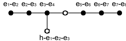
FIGURE 5. \mathbb{A}_3 \oplus \mathbb{A}_3 \subset \mathbb{E}_8
