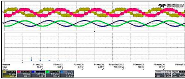
(c) SPOD: M = 0.9 - f_{sw} = 10 kHz
