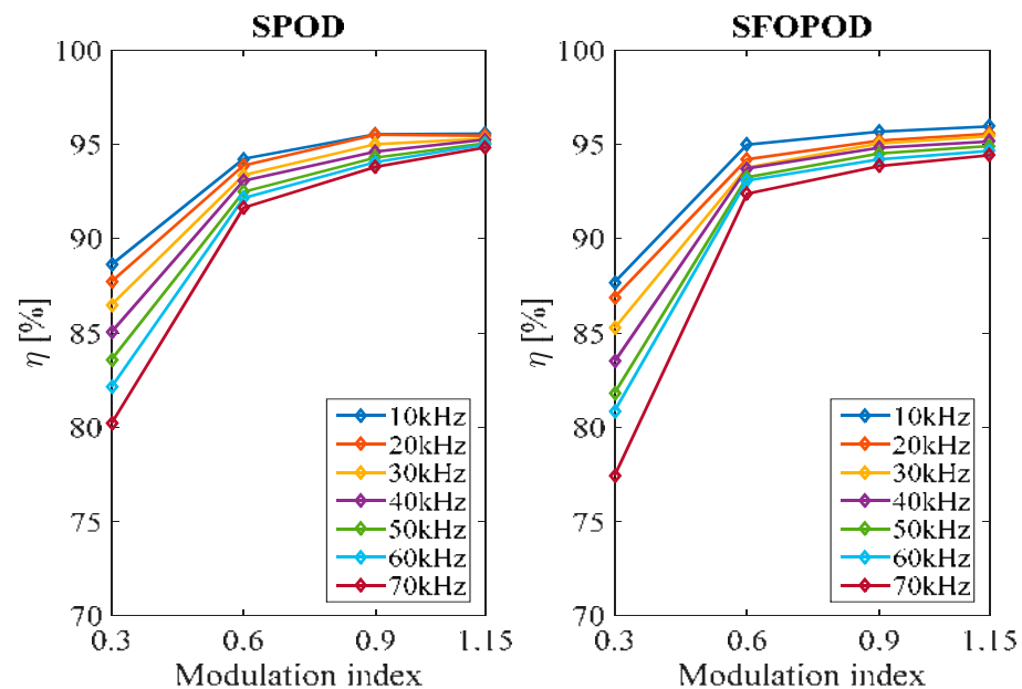
Figure 21. Experimental conversion efficiency trends of SPOD and SFOPOD schemes.
