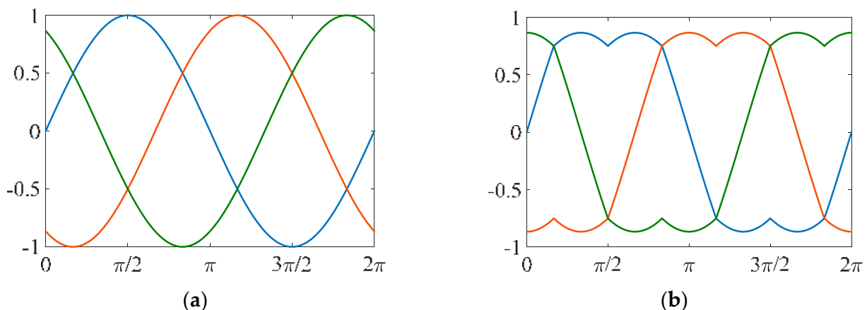
Figure 4. Modulation signals with modulation index equal to 1: (a) sinusoidal; (b) Switching Frequency Optimal—SFO.
