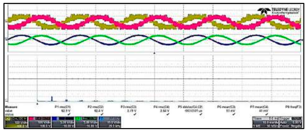
(e) SAPOD: M = 0.9 - f_{sw} = 10 kHz
