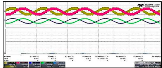
(b) SFOPD: M = 0.9 - f_{sw} = 40 kHz
