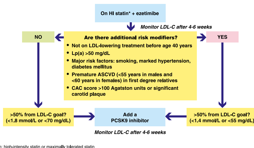
Fig. 2. Algorithm for managing high LDL-C levels in FH patients without ASCVD.
