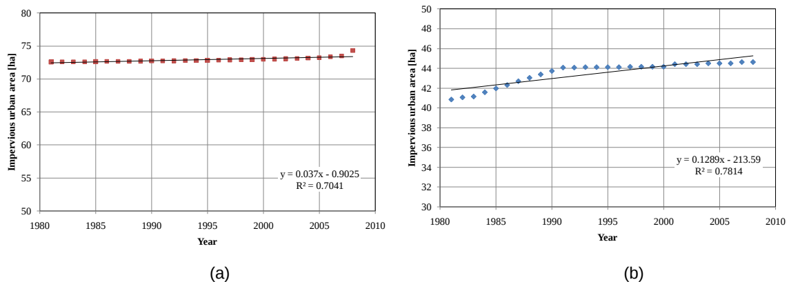
Figure 5. Linear trend of impervious area for Montelepre (a) and Giardinello (b)
