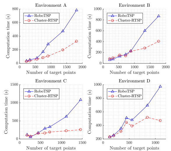
Fig. 8. Computation time for problem instances shown in Fig. 6.
