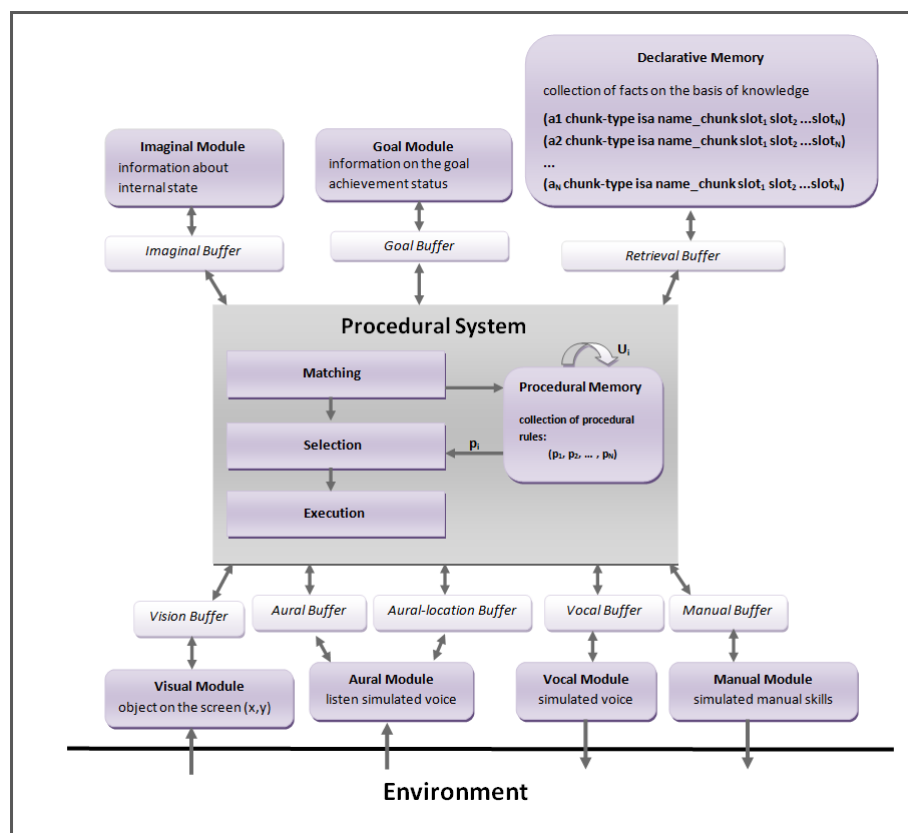
Figure 1. A representation of the ACT-R architecture.
