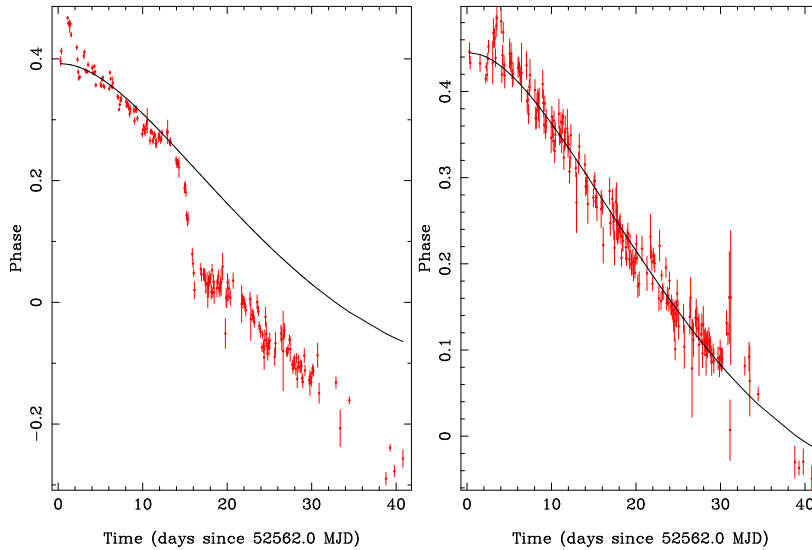
Fig. 1 Left: Phase vs. time for the fundamental of the pulse frequency of SAX J1808.4-3658. Right: Phase vs. time for the first harmonic of the pulse frequency of SAX J1808.4-3658. On top of the data, the best-fit function (including both the spin-up due to accretion and the spin-down at the end of the outburst) is plotted as a solid line (from [29]).
